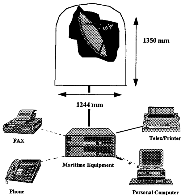
Figure 3-9. Inmarsat A and B Standard Configuration. After Ref [14].
