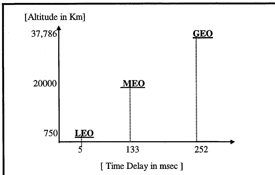
Figure 1.1 Satellite Altitudes vs. Time Delay. "After Ref. [2]."
