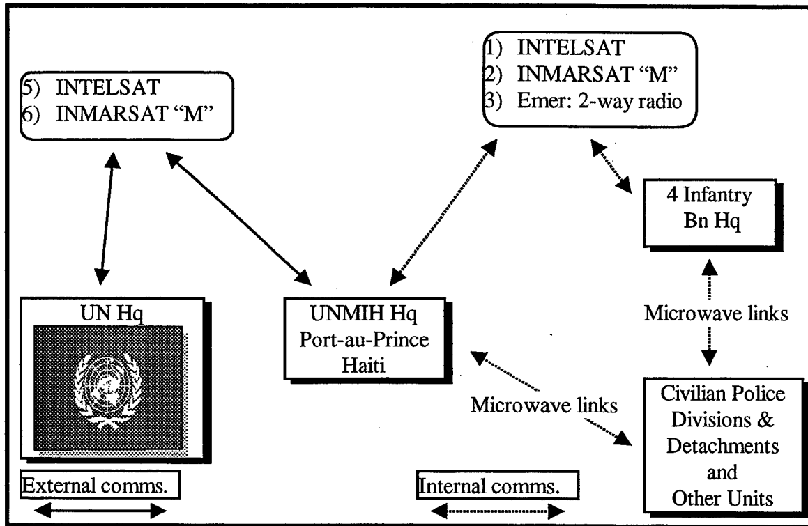
Figure 7.1 The UN Mission Static Communications Network
