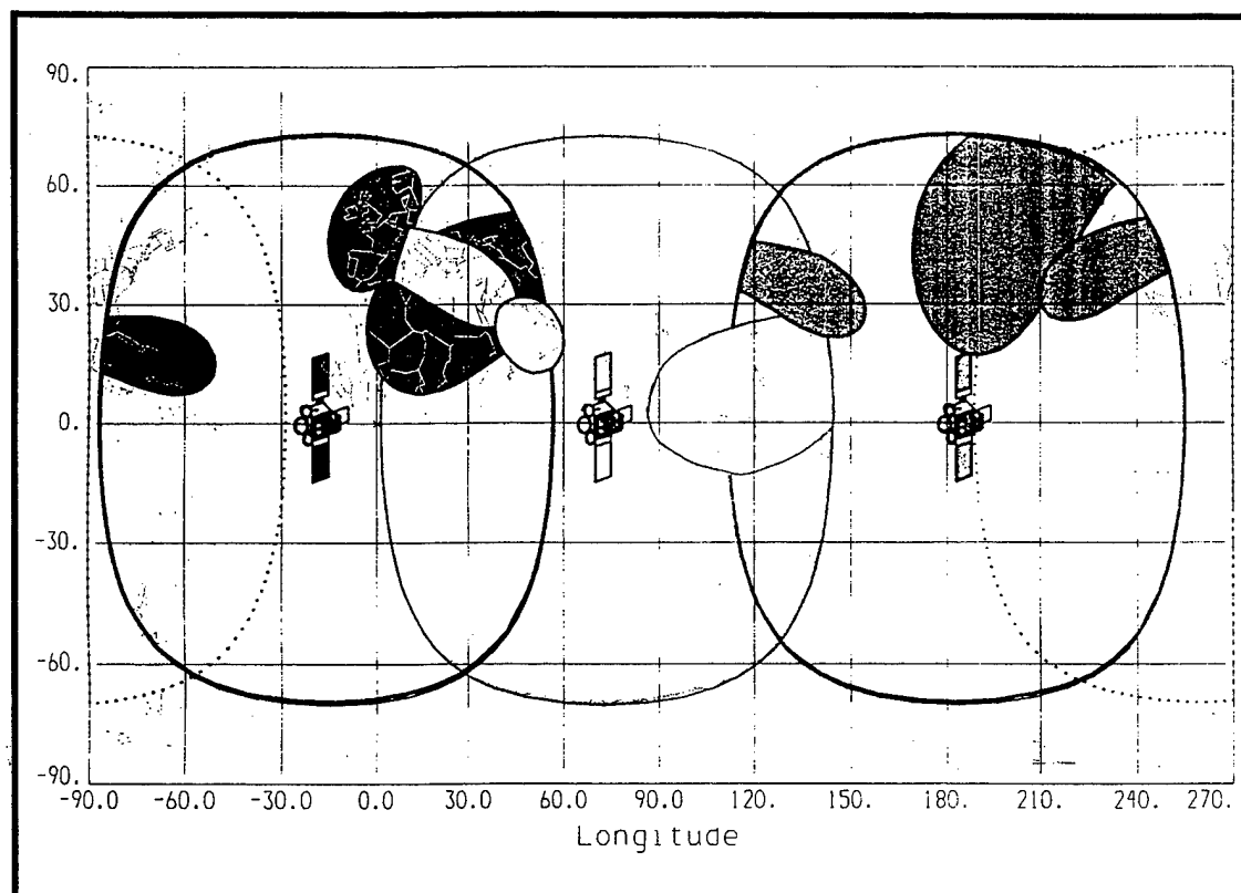
Figure 4.5 The GBS/UFO (Phase II) Coverage “From Ref. [25].”
