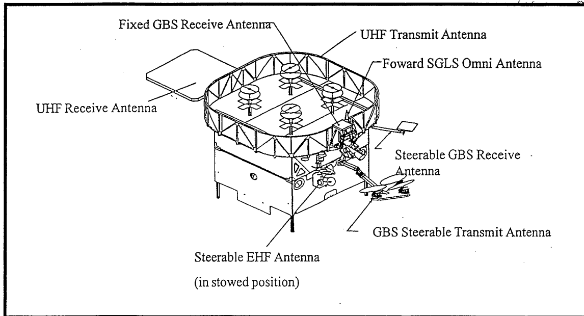
Figure 4.4 The GBS/UFO Satellite "From Ref. [25]."
