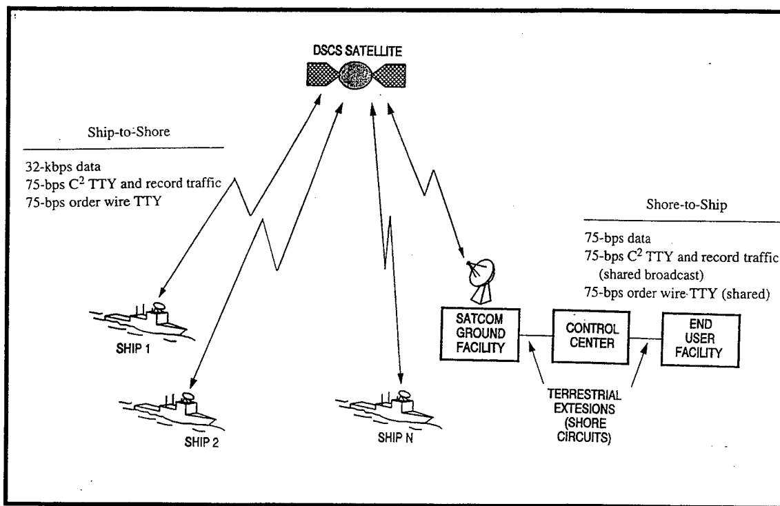
Figure 3.6 US Navy DCSC Connectivity and Capabilities "From Ref. [19]."
