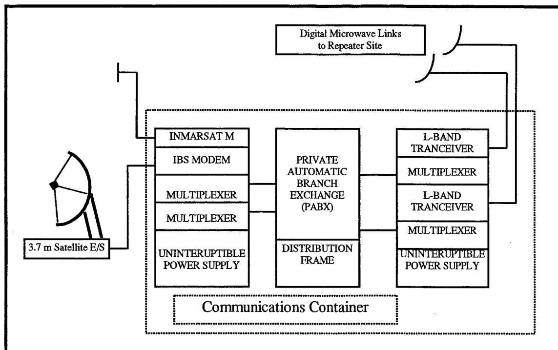
Figure 7.3 Battalion Headquarters Satellite Node Earth Station “After Ref.[35].”
