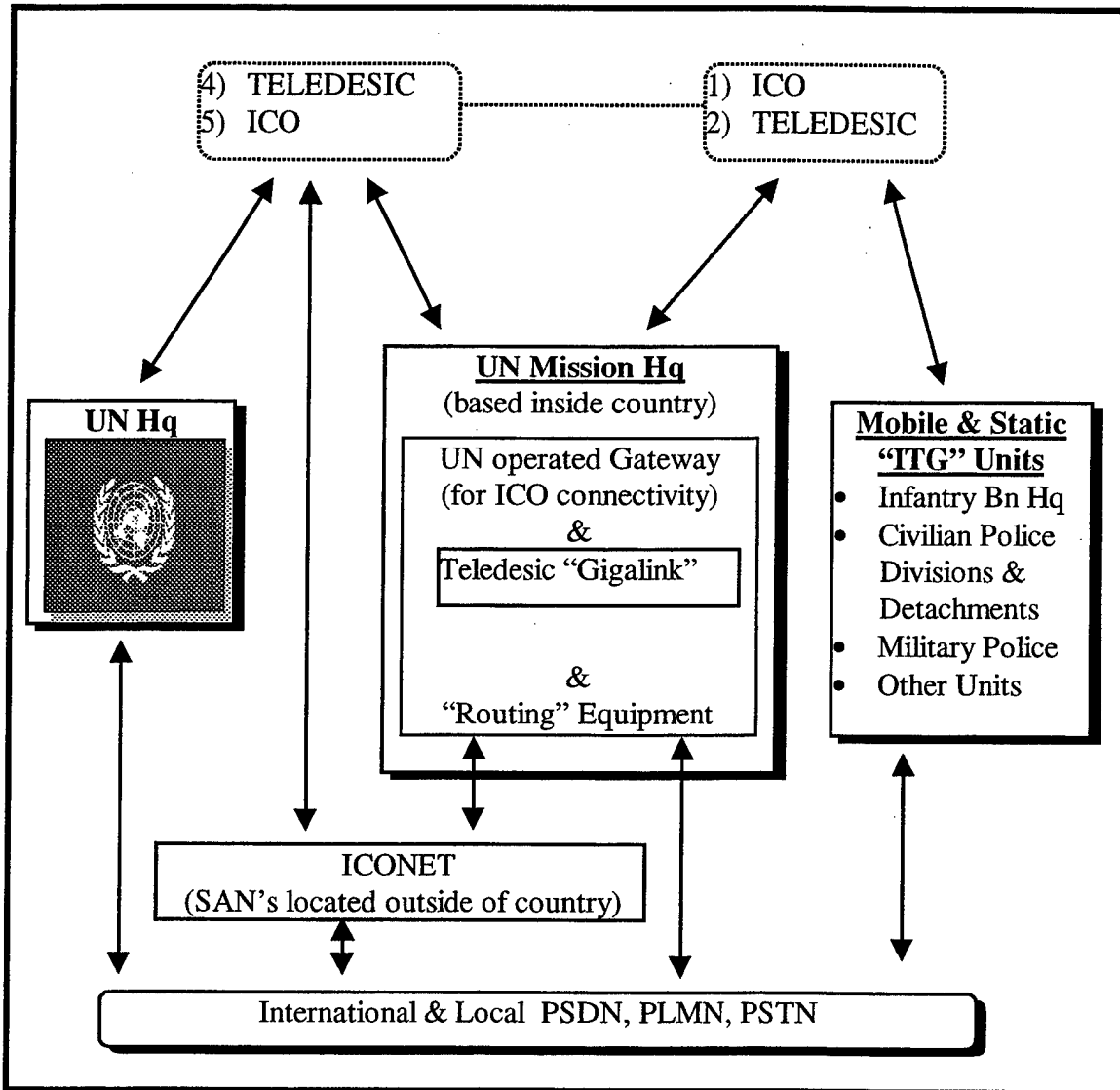
Figure 7.5 The "ITG" Communications Network for UN peacekeeping
