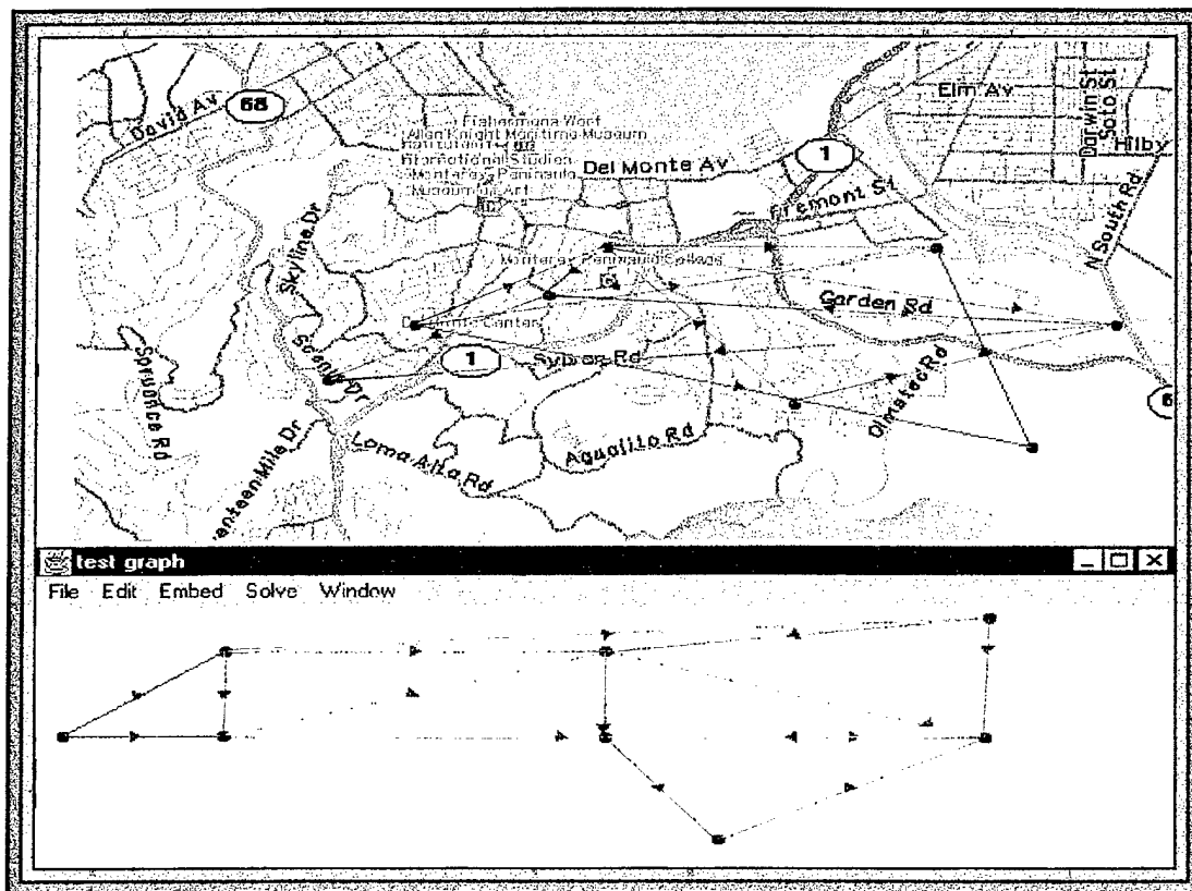
Figure 10: A new node and two new arcs added to figure (9). The new arcs connect the new node to nodes 1 and 4 and are identified on both displays by the highlighted arcs.
