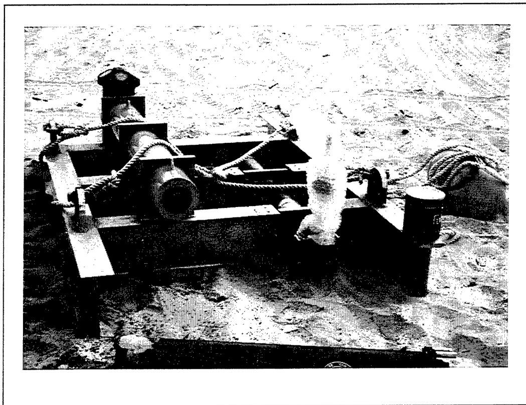
Figure 6. ADCP deployed in equipment mount (photo by T. E. White)
