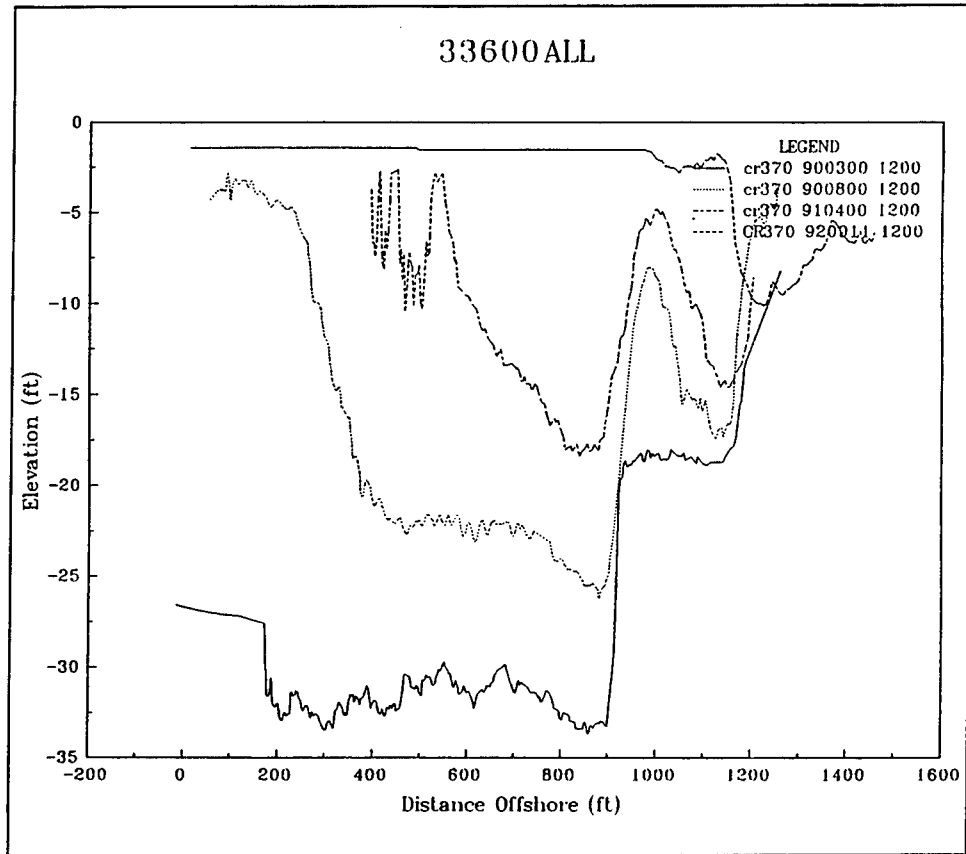
Figure 20. Example of impoundment basin surveys
