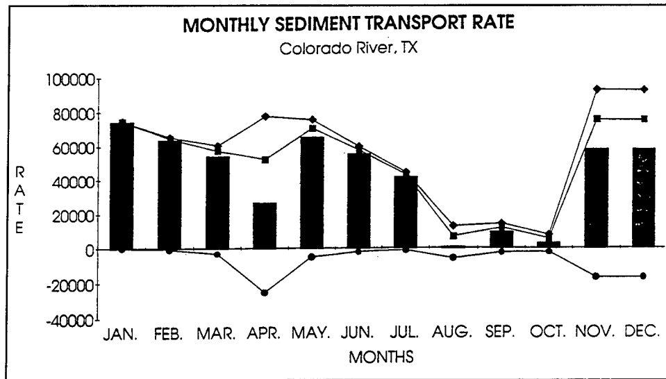
Figure 26. Monthly sediment transport rate, in cubic meters per month. Squares are the gross transport to the southwest, circles are the gross transport to the northeast, diamonds are total gross transport, and bars are the net transport. Calculated by SPM method
