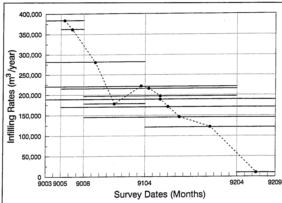
Figure 27. Plot of impoundment basin infilling rates
