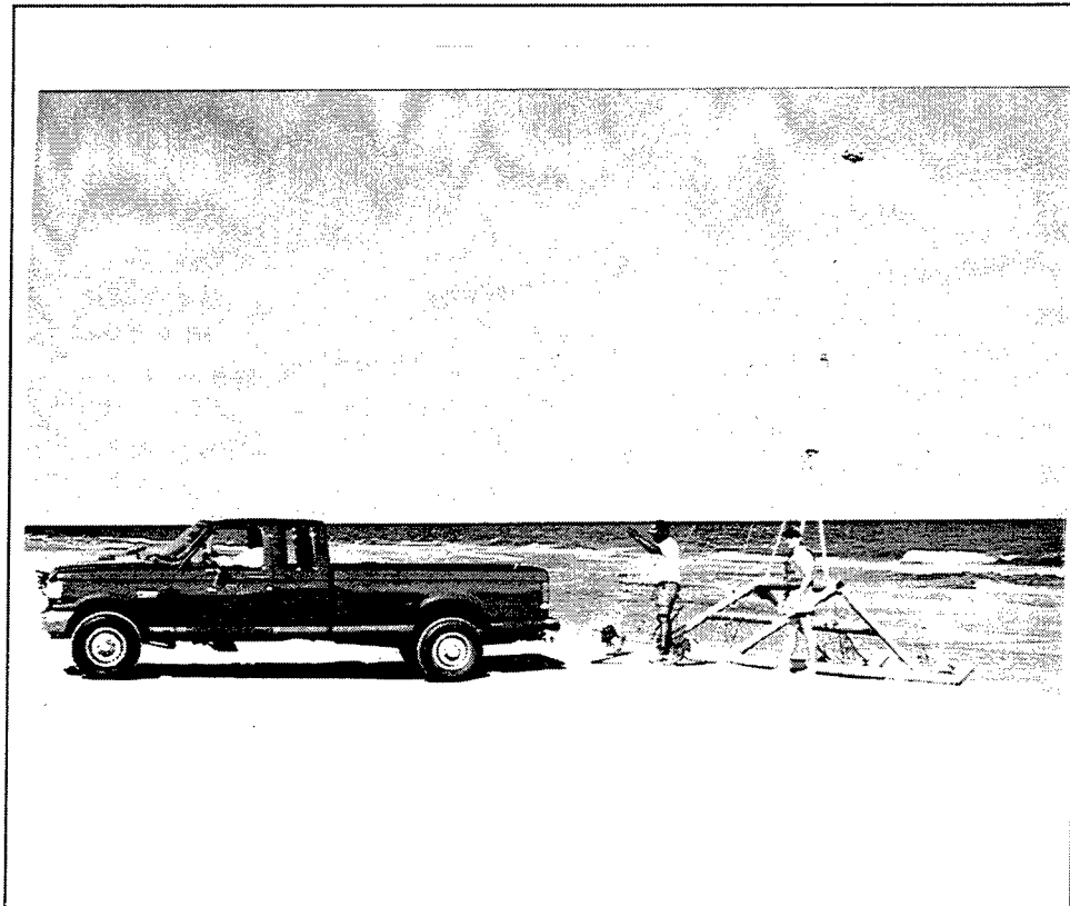
Figure 10. Rod setup for offshore geodimeter surveying (photo by T. E. White)
