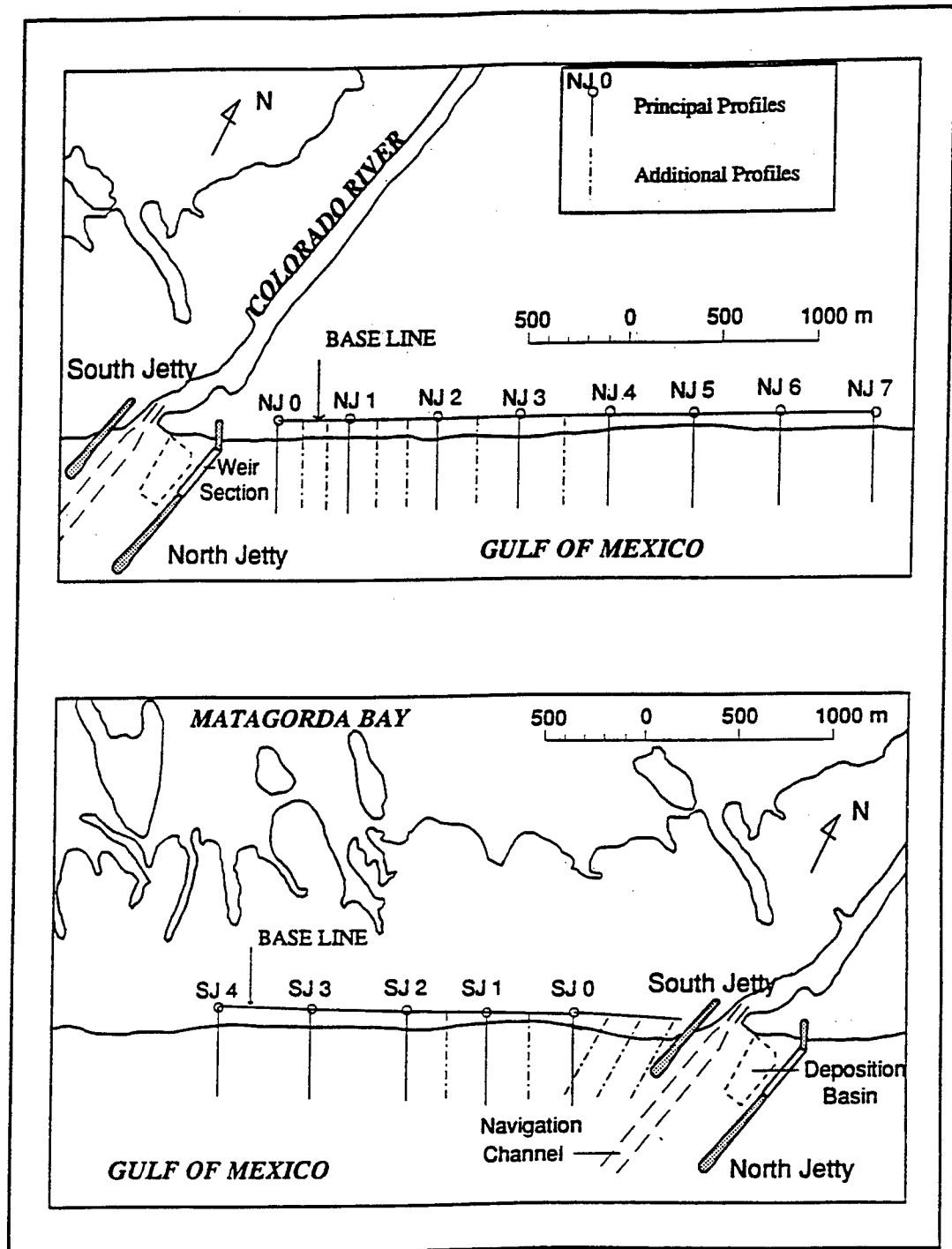
Figure 9. Survey line locations (from Liang1995)
