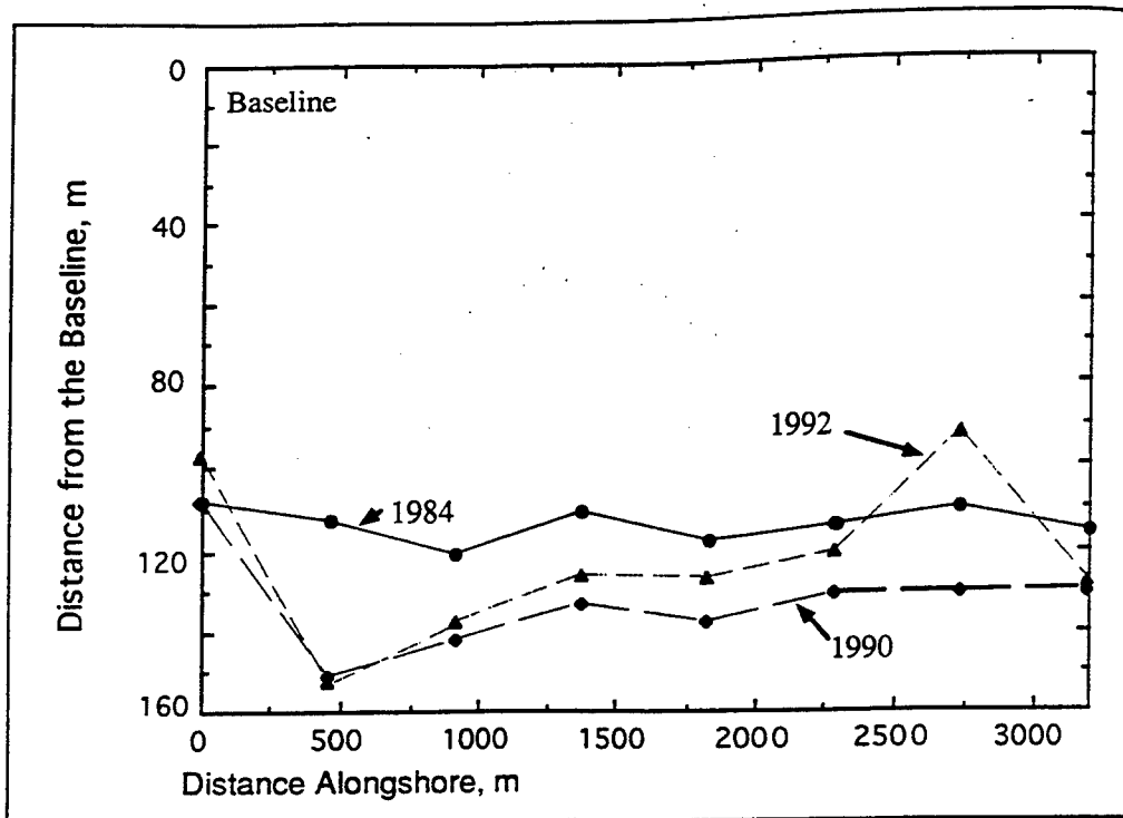
Figure 19. Shoreline positions northeast of the mouth of the Colorado River between 1984 and 1992. Longshore distances are from NJO. (from Liang 1995)
