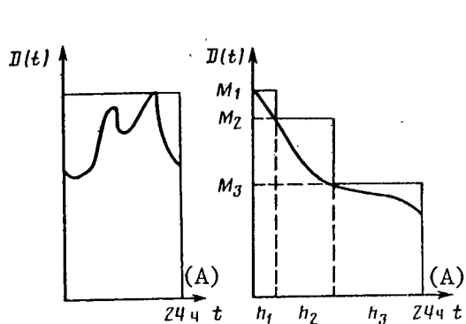
Figure 1. Daily Load Schedule.
