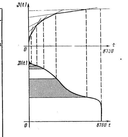
Figure 4. Graph of the Broken Line z(t) and Graph of the Duration of the Load D(t) .
