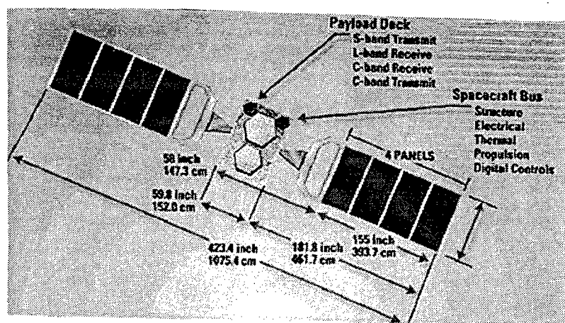
Figure 4.6. GLOBALSTAR Satellite
