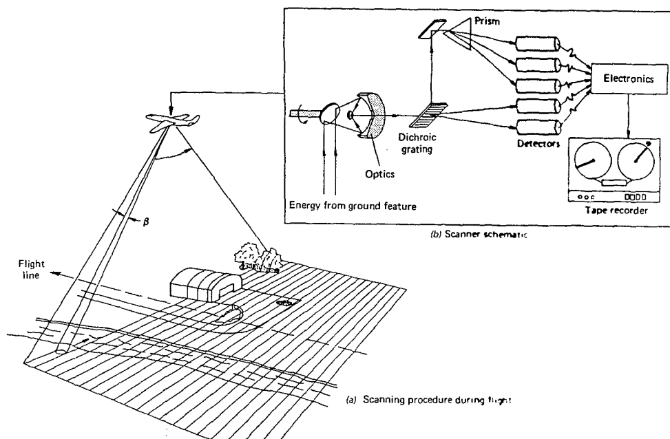
Figure 7.7. Across Track Scanner on an Aircraft Platform [Lillesand, 1994].
