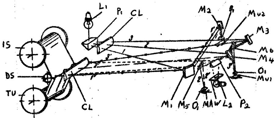
Fig. 8 Optical diagram of the RNVU instrument. L_1 -- lamp of pendulum illuminator, L_2 -- lamp of time marker illuminator, P_1 -- prism, C -- condenser lens, M_1 -- M_6 -- reflecting mirrors, P_2 -- time marker prism, B -- blind of slit time marker of relay type, M_{i1} , M_{i2} -- mirrors of inclination-measuring pendulums, MA -- mirror of vertical accelerometer, O_1 -- objectives, CL -- cylindrical lens, DS -- drive shaft, IS -- idler spool, TU -- takeup spool.
