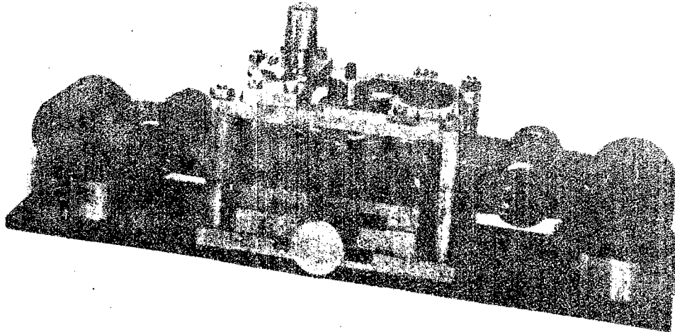
Fig. 7 Overall view of inclination-measuring accelerometer.
