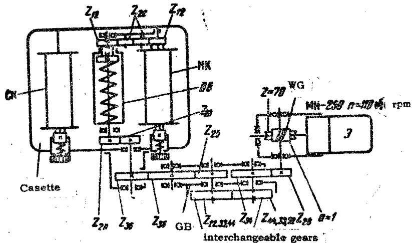
Fig. 9 Kinematic diagram of the RNVU instrument. E -- electric motor, WG -- worm gear, DS -- driving shaft, IS -- idler spool, TJ -- takeup spool, GB -- gear box, Z -- gears.
