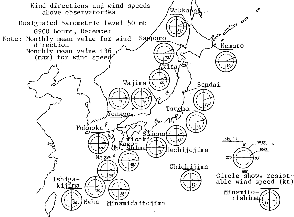
Figure 22. Wind Directions and Wind Speeds Above Observatories (Winter)
