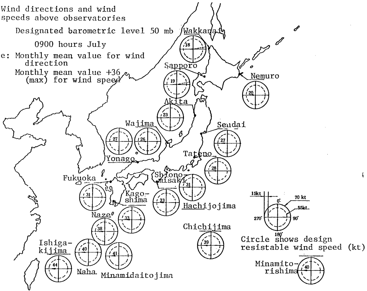
Figure 23. Wind Directions and Wind Speeds Above Observatories (Summer)
