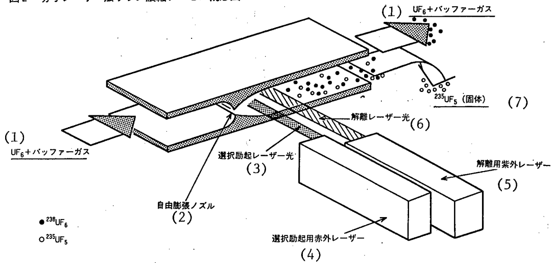
Figure 2. Schematic Diagram of Uranium Enrichment Process by Particle Laser Method
