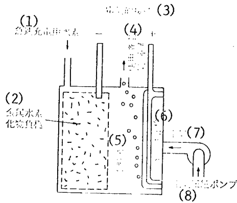
Figure 9. Hydrogen/Hybrid-Air Battery Amenable to Charging Like Usual Secondary Batteries as Well as Charging by Means of Hydrogen Gas
