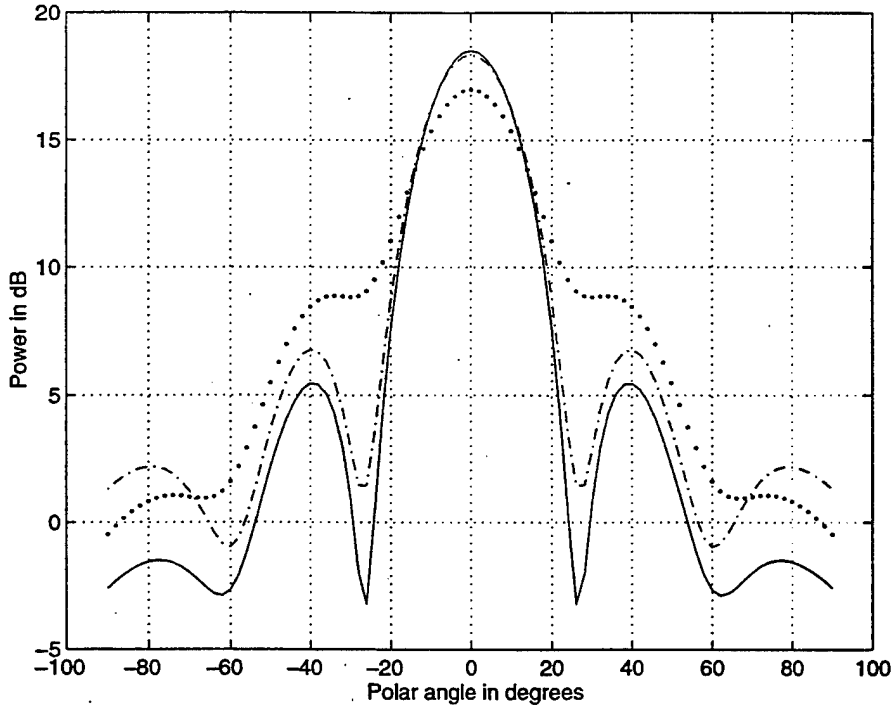
Figure 24: Patterns for arrays with a curved ground plane (dotted: without phase corrections; dash-dot: with phase corrections) and a flat array (solid).
