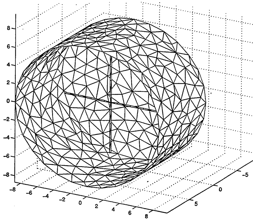
Figure 16: Cavity-backed crossed dipole antenna.
