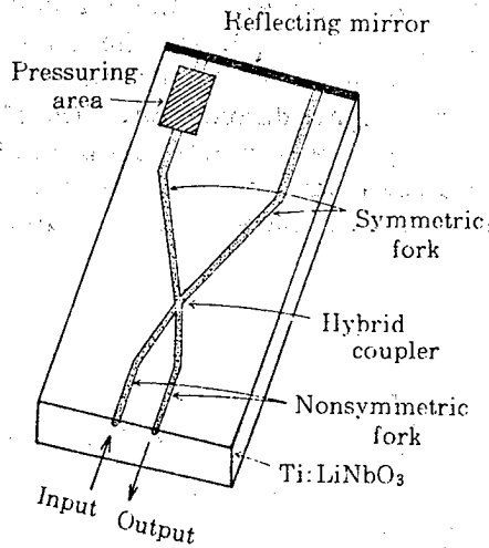
Figure 3. Pressure Sensor Using \text{LiNbO}_3 X-Forked Waveguide 5
