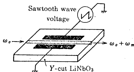
Figure 8. Serrodyne-Type SSB Modulator 16
