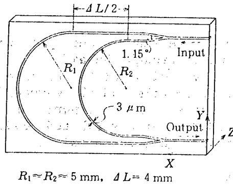
Figure 2. High-Sensitivity Temperature Sensor Being Proton-Exchanged \text{LiNbO}_3 \pi -Arced Waveguide 3
