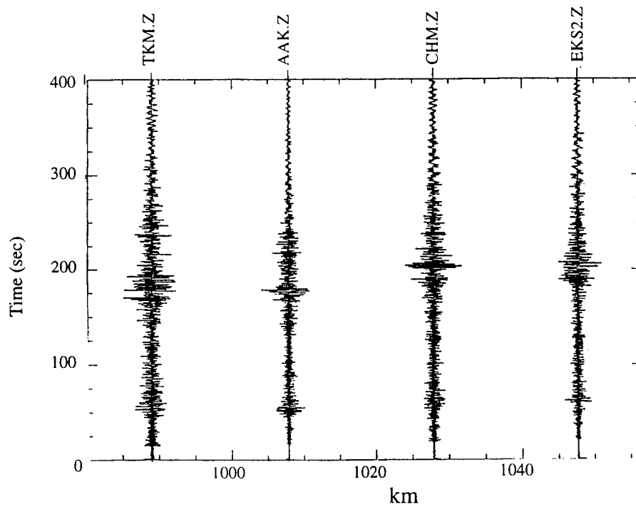
Figure 11a: Record section of plot event #2 in figure 7a, 27 June 92. Data was bandpassed filtered 1-5 Hz. The Lg coda varies across the array.
