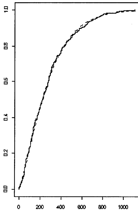
Empirical and Hypothesized weibull CDFs
