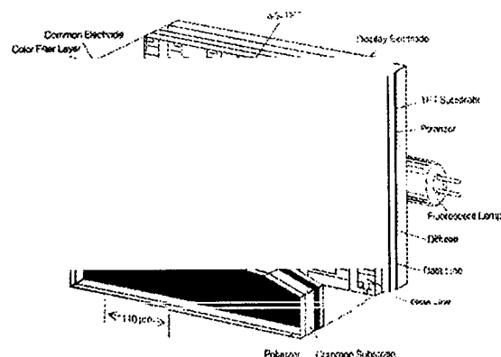
FIGURE A-3: Cross-Section of Active Matrix Liquid Crystal Display
