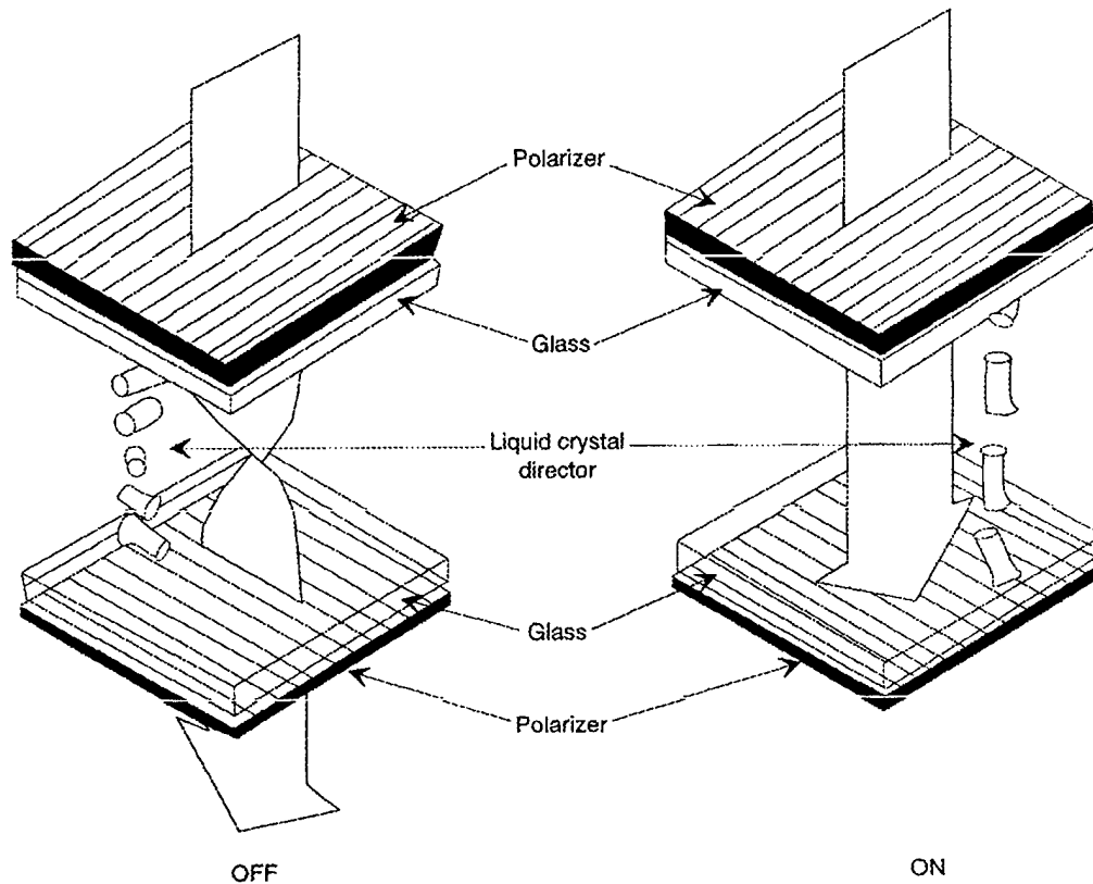
FIGURE A-1: Twisted Nematic Liquid Crystal Cell
