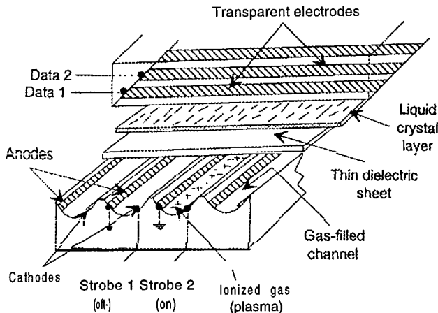
FIGURE A-5: Plasma Addressed Liquid Crystal Display
