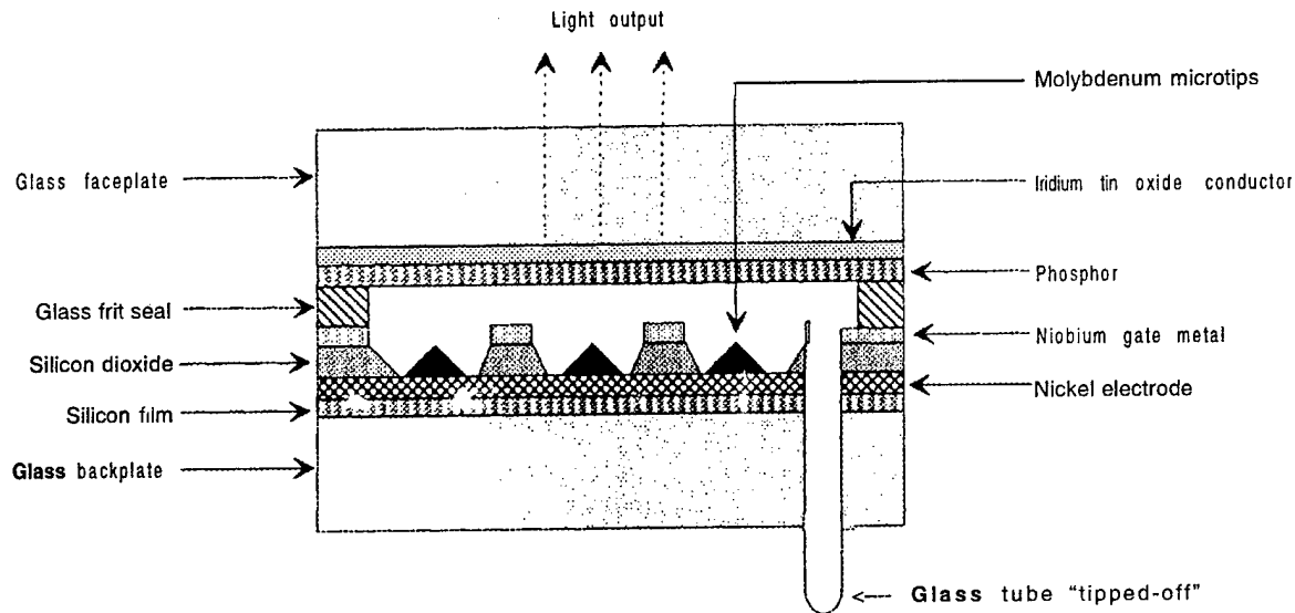
FIGURE A-6: Field Emission Display Microemitter
