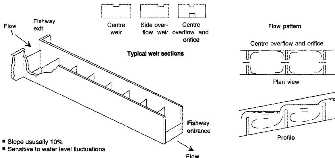
FIGURE 3-1: Weir Fishway
