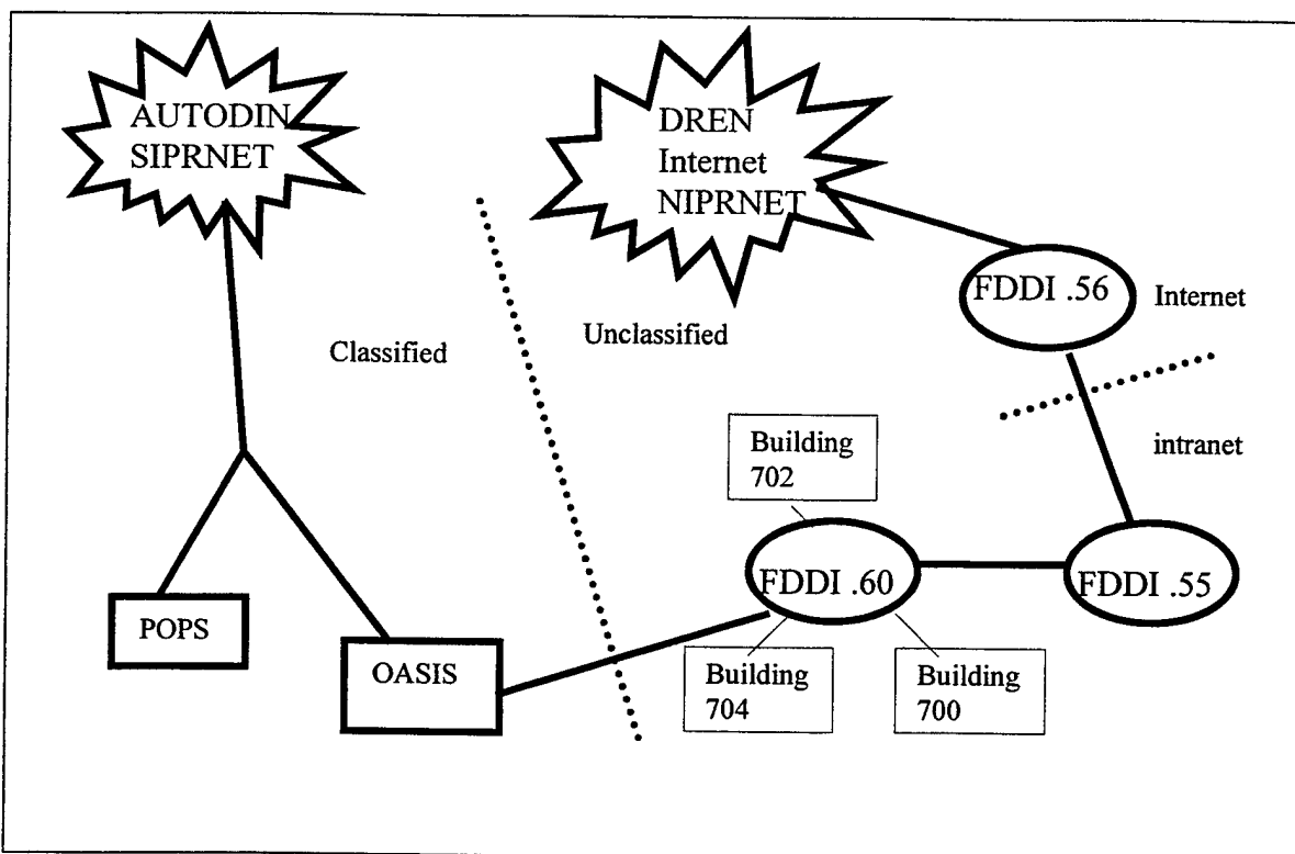
Figure 4-2. FNMOC LAN Configuration
