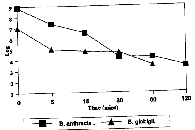
Figure 5. Glutaraldehyde (5%)
