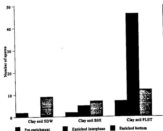
Fig 5. The effect of enrichment and biphasic separation on the concentration of spores of Bacillus anthracis in environmental samples.
