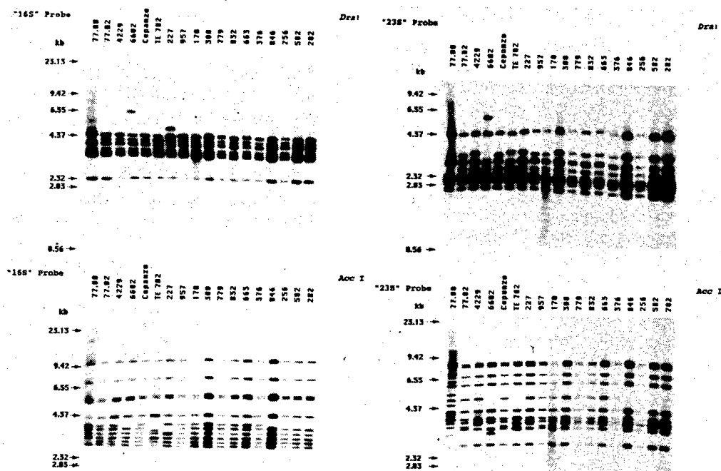
Figure 1. Southern blot of genomic DNA of avirulent and virulent Bacillus anthracis strains cleaved by DraI (upper part) or AccI (lower part) and probed with 32 P labelled 16S-493 (left) or 23S-508 (right) rDNA sequences. The Bacillus anthracis strains: 77.00, 77.02, 4229, 6602, Cezanzo and 957 were pXO1 + or/and pXO2 - . The Bacillus anthracis strains: 227, 170, 300, 779, 932, 663, 376, 846, 256, 582 and 282 were pXO1 + and pXO2 + .
