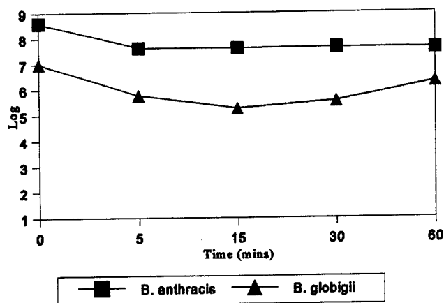
Figure 10. Tegodor (1%)
