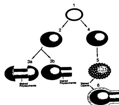
Figure 2. Diagrammatic representation of Bacillus anthracis spore germination and outgrowth. Events (1, 2, 3a and 3b) depicted on left side represent incubation in fortified beef heart infusion and staining with EAI 6G6 monoclonal antibody - FITC conjugate. Events (1, 4, 5 and 6) depicted on the right side represent incubation in fortified beef heart infusion supplemented with 50% heat-inactivated horse serum and 0.8% sodium bicarbonate and staining with FDF-1B9 monoclonal antibody-FITC conjugate.
