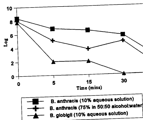
Figure 1. Chlorox
