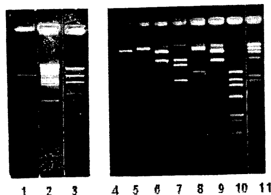
Fig 1. Restriction profiles of hybrid plasmid pSP19/91 with B. anthracis cap operon 1,4-pSP19/91, restricted with Bam HI; 3, 11-DNA of phage 1 restricted with Hind III, 5-10-pSP 19/91, restricted with SacI , Bgl II, Hind III, SacI + SalI , SalI + Bgl II, Hind III+ Eco RI.
