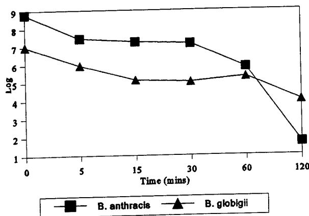
Figure 4. Glutaraldehyde (2%)
