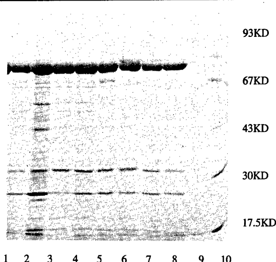
Figure 4: Protein profiles of the strains of B. anthracis
