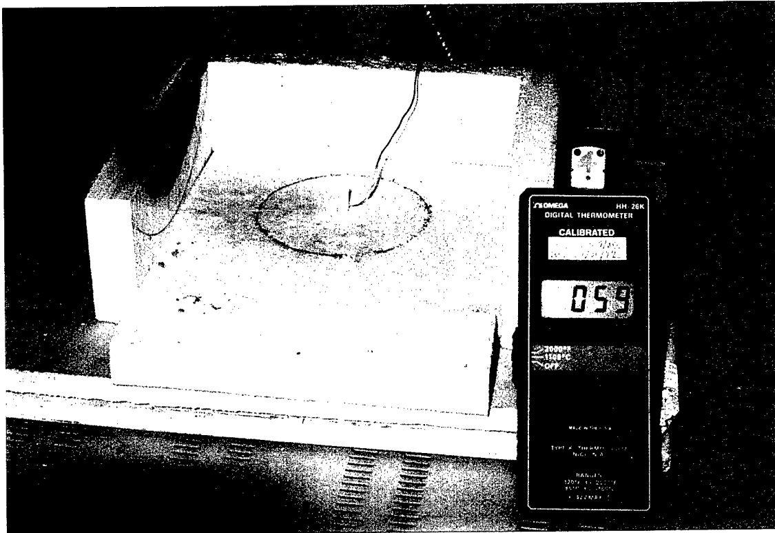
Figure 19. Temperature measurement of distal end of YbAG/YAG SELP in the electric furnace test .
