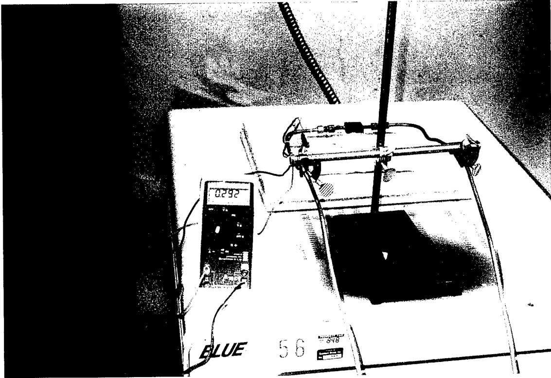
Figure 17. GaSb PV cell power evaluation of YbAG/YAG SELP PV using high temperature electric furnace as the heat source.
