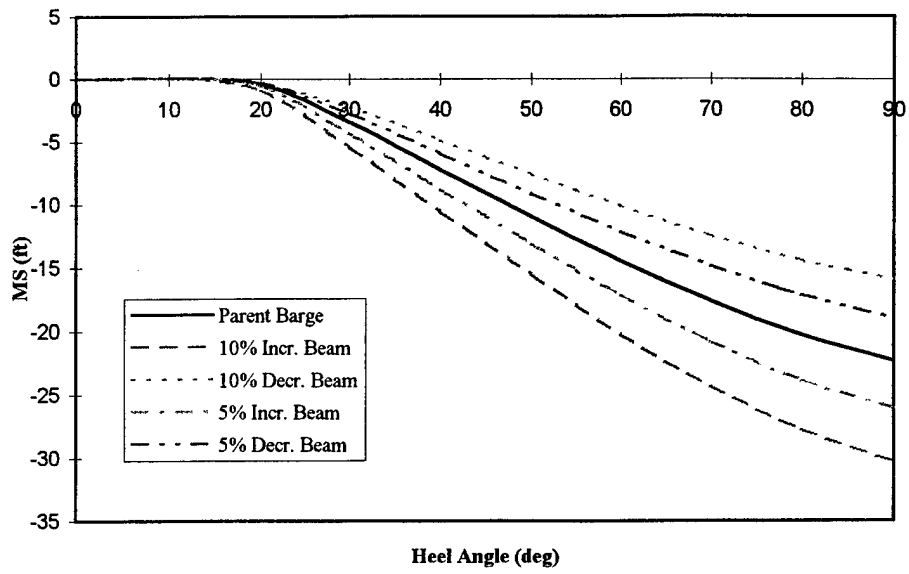
Figure 13. Residuary Stability for Changes in Beam (Barge 2)
