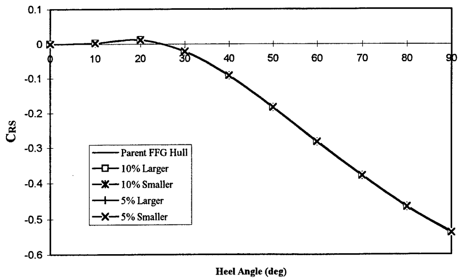
Figure 27. Residuary Stability Coefficient for "Geo-Sim" FFG-7
