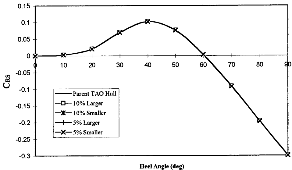
Figure 28. Residuary Stability Coefficient for "Geo-Sim" T-AO
