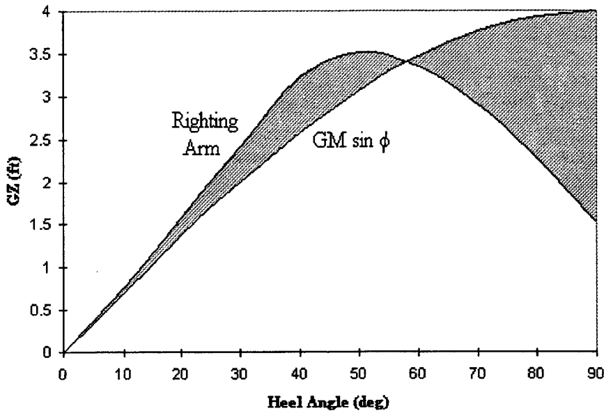
Figure 8. Residuary Stability Contribution
