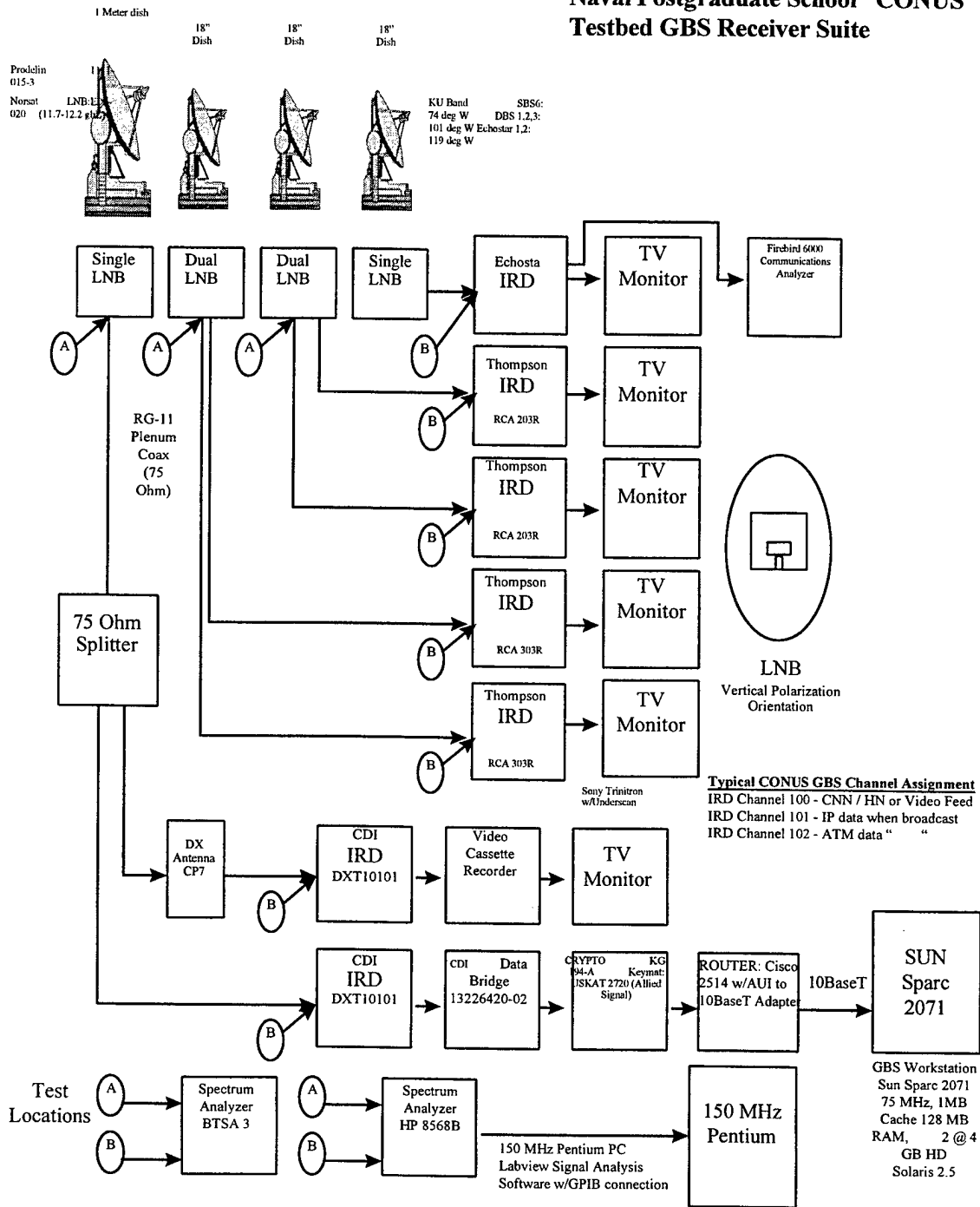
Figure 8 GBS CONUS Testbed Receive Suite
