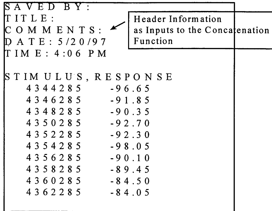
Figure 24 Output Data File with Header Information
