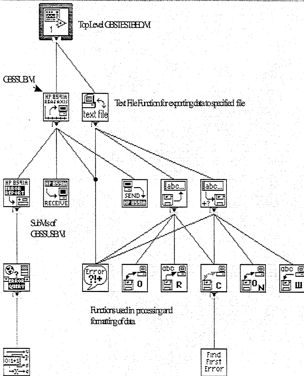
Figure 23 VI Hierarchy
