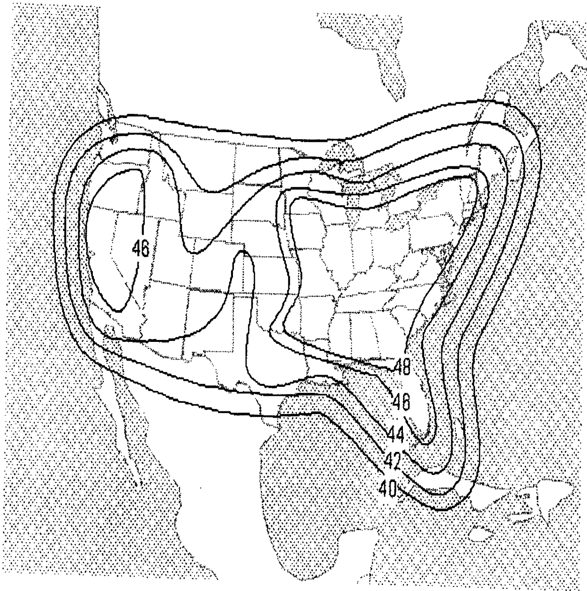
Figure 4 EIRP Coverage of SBS-6 Satellite
