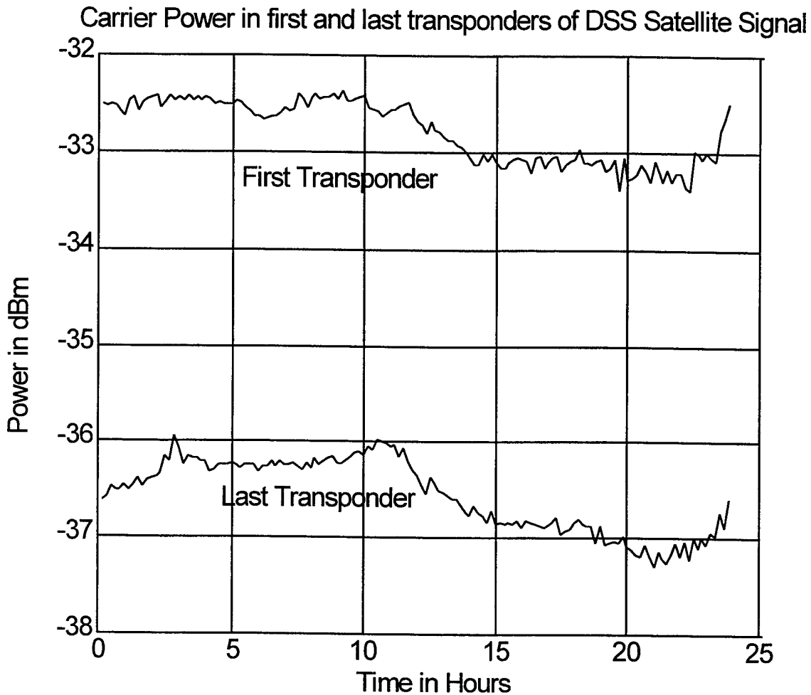
Figure 26. Carrier Power for DSS Channel 1 and 16 of the DSS Satellite Signal
