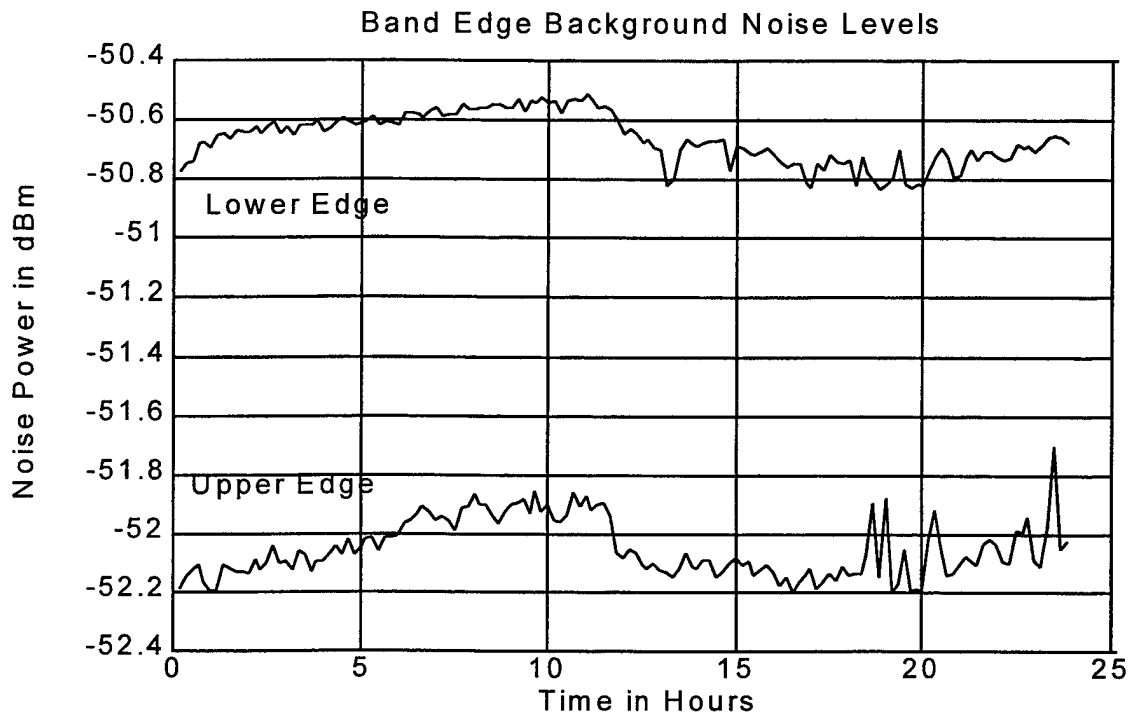
Figure 33. Background Noise Levels for the Hughes SBS-6 Satellite Signal
