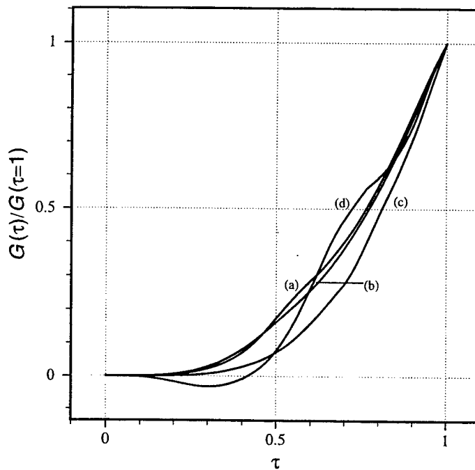
Figure 26. Normalized gain along the undulator G(\tau)/G(\tau = 1) for electron beams with radius (a) \sigma_e = 0.2 , (b) \sigma_e = 0.45 , (c) \sigma_e = 0.9 , and (d) \sigma_e = 1.6 . Rayleigh length and mode waist radius same as in Figure 25.
