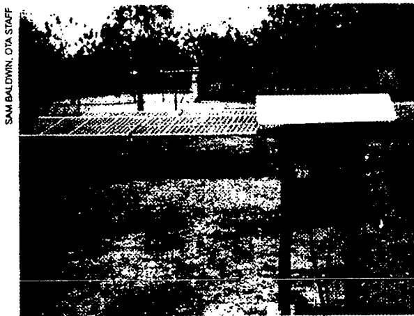
A photovoltaic pumping system near Ziniare, Burkina Faso. This system provides clean drinking water, reduces the labor of lifting and hauling water, and can help break waterborne disease cycles.
