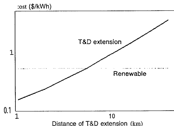
FIGURE 5-4B: Cost-Effectiveness of T&D Extension and PVs, by Length of Grid Extension
