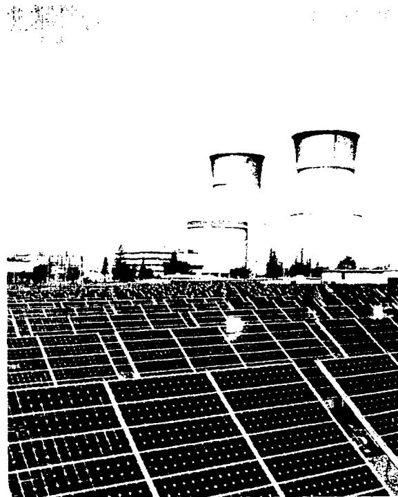
The Sacramento Municipal Utility District (SMUD) 2-MW photovoltaic plant is sited at the site of the now closed Rancho Seco nuclear power plant.
