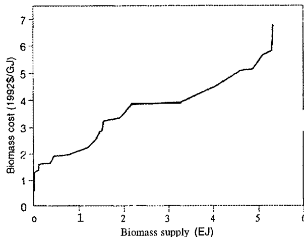
FIGURE 2-2: Supply Curve for Whole Tree Chips
