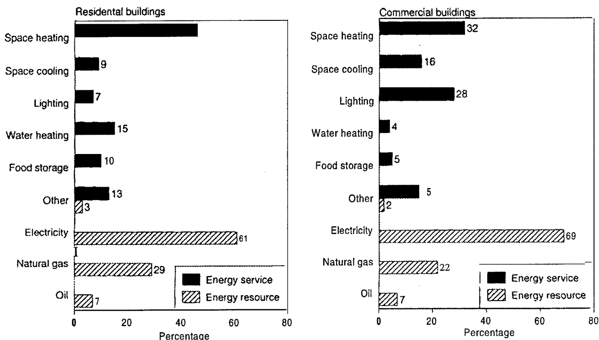
FIGURE 3-3: Energy Services and Supplies in U.S. Residential and Commercial Buildings
