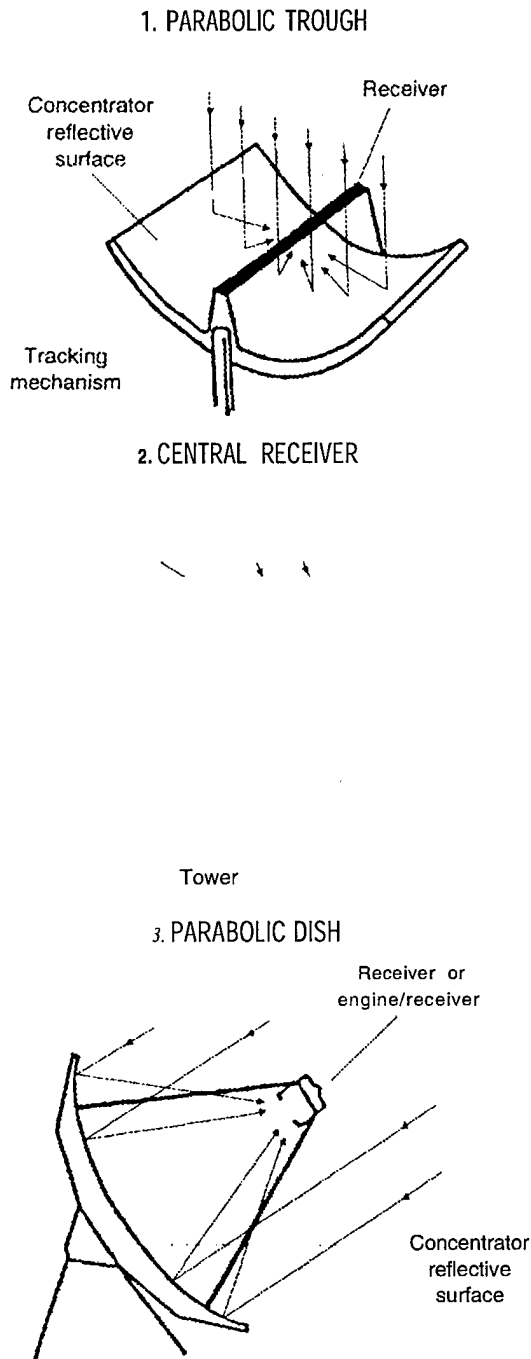
FIGURE 5-2: Solar Thermal Collectors
