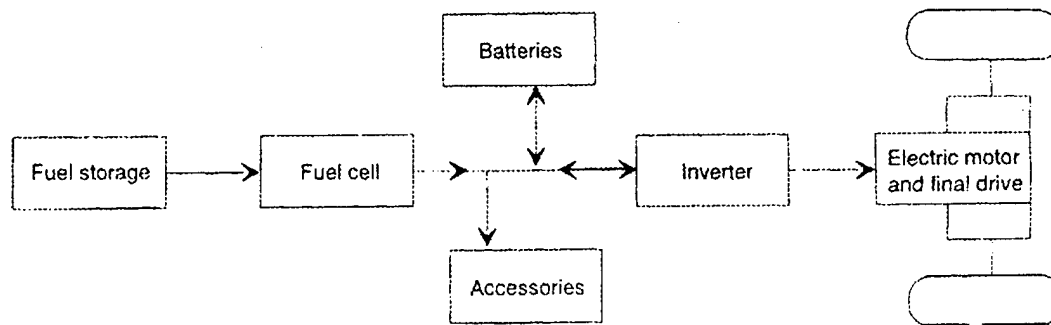
FIGURE 4-4: Advanced Fuel Cell Vehicle Power Train Configuration
