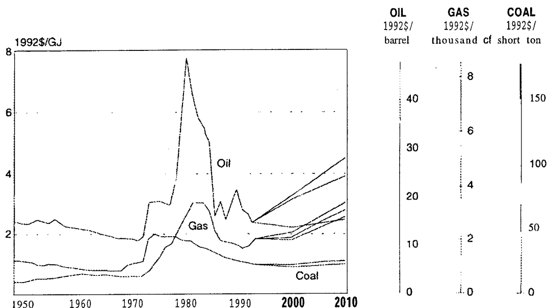
FIGURE 1-A-4: Historical and Projected Fossil Fuel Prices
