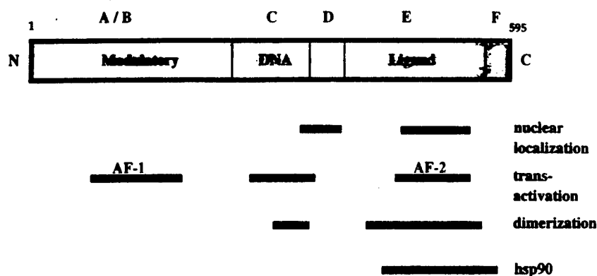
Figure 2. Schematic representation of the human estrogen receptor showing several functional domains and associated activities.
