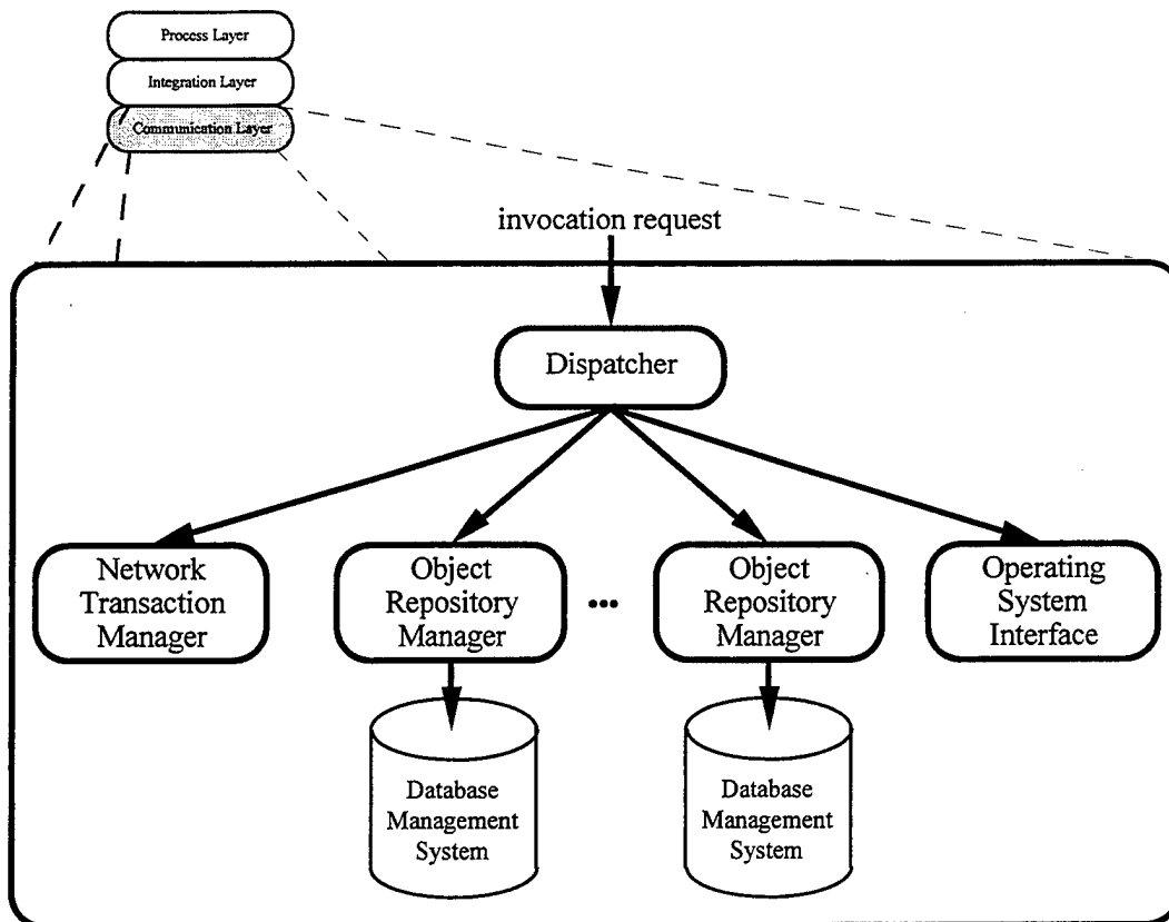
Figure 10 Communication Layer
