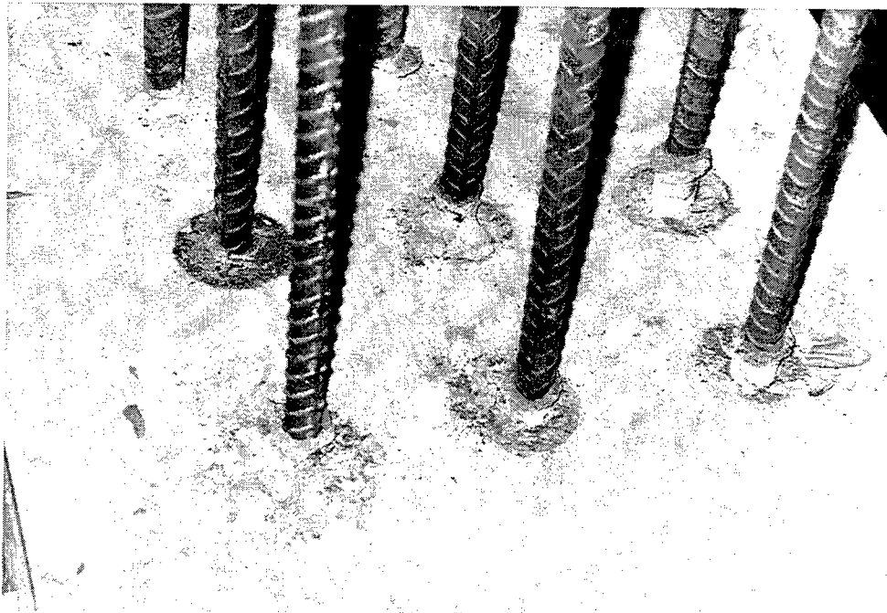
Figure 25. Typical material fracture normally occurring during anchor failure
