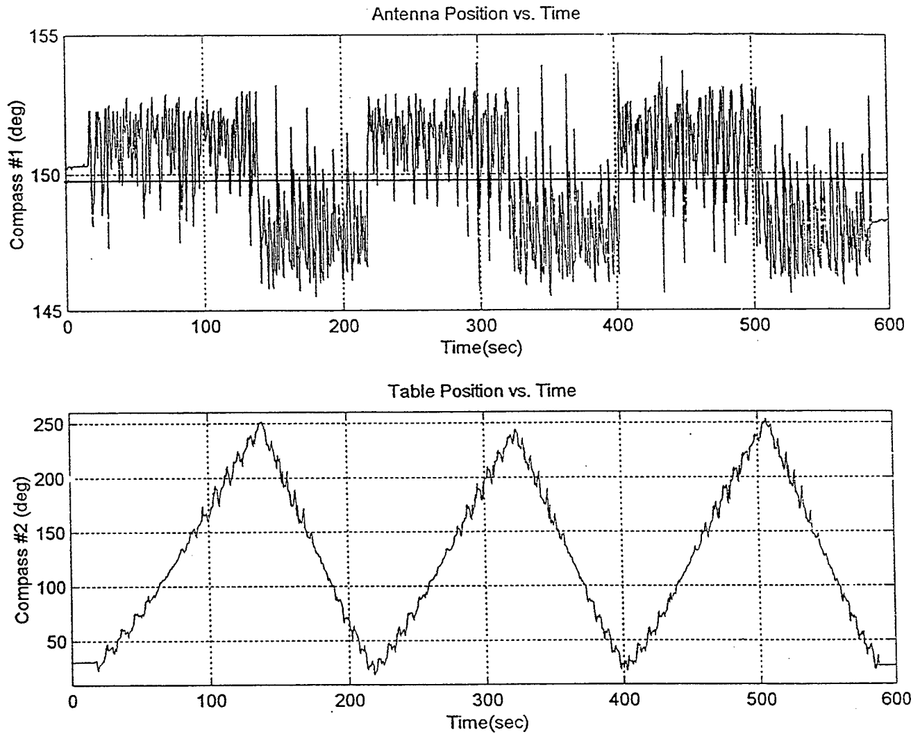
Figure 6: Top plot shows antenna orientation versus time for the table orientations shown in the lower plot. The fixed reference direction is the straight line at 149.7°. Table rotation speed is 2°/sec.
