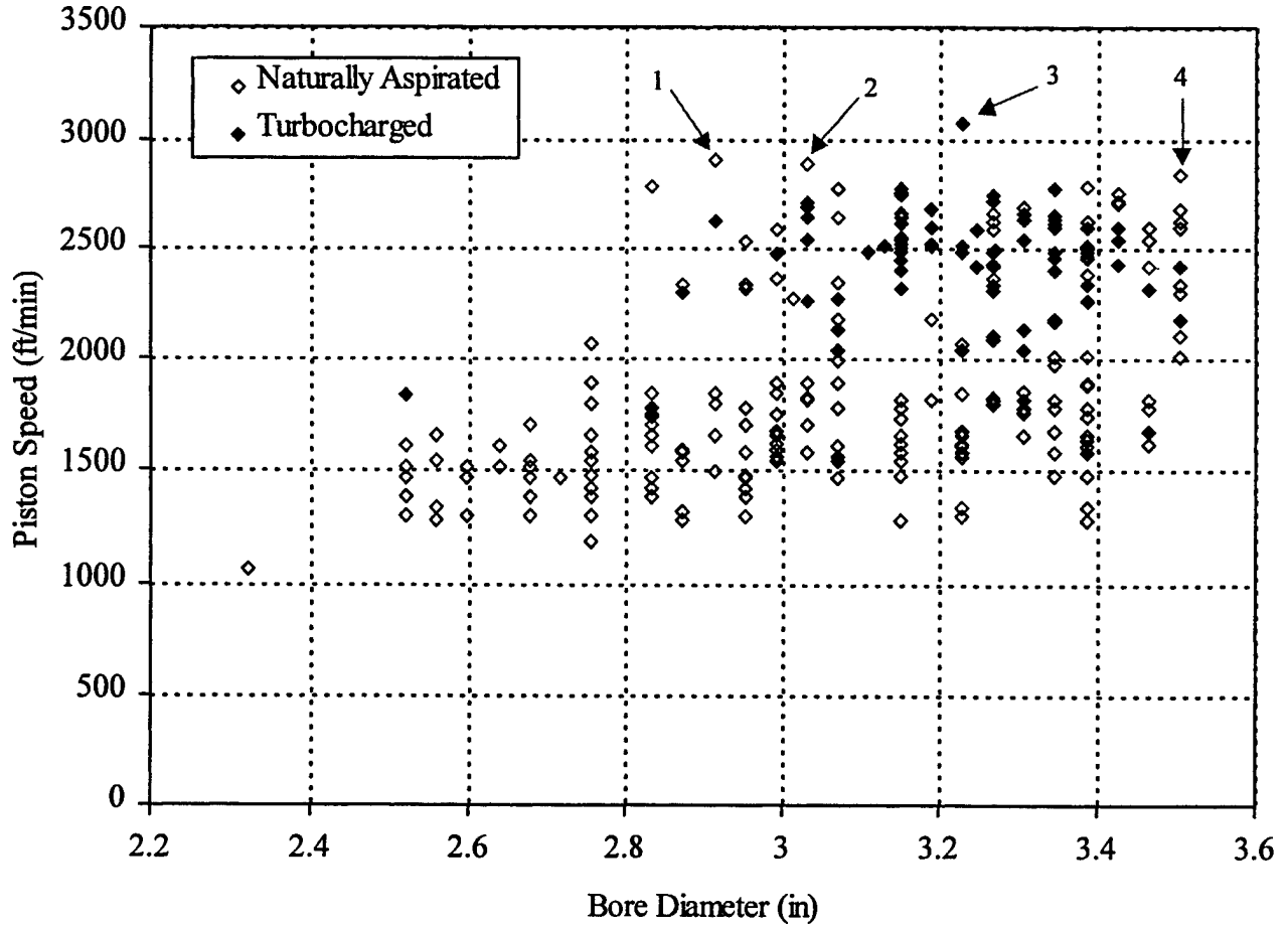
Figure E-3. Piston Speed at Rated Horsepower vs. Bore Diameter
