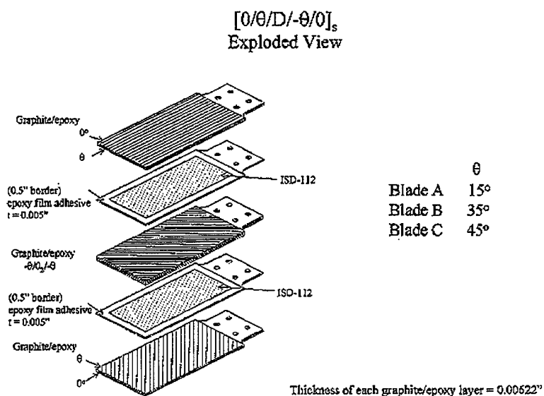
FIGURE 31. Damped Blade
