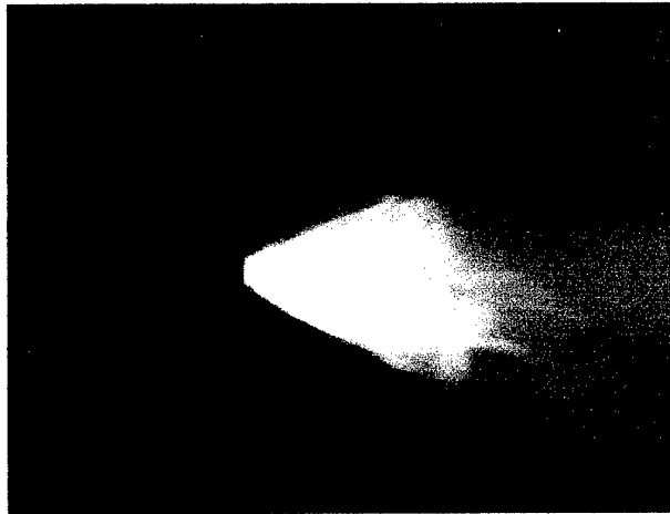
Fig.2.4. Appearance of a discharge with the model with conic frontal part. M = 2.3, I = 1.6 \text{ A}
