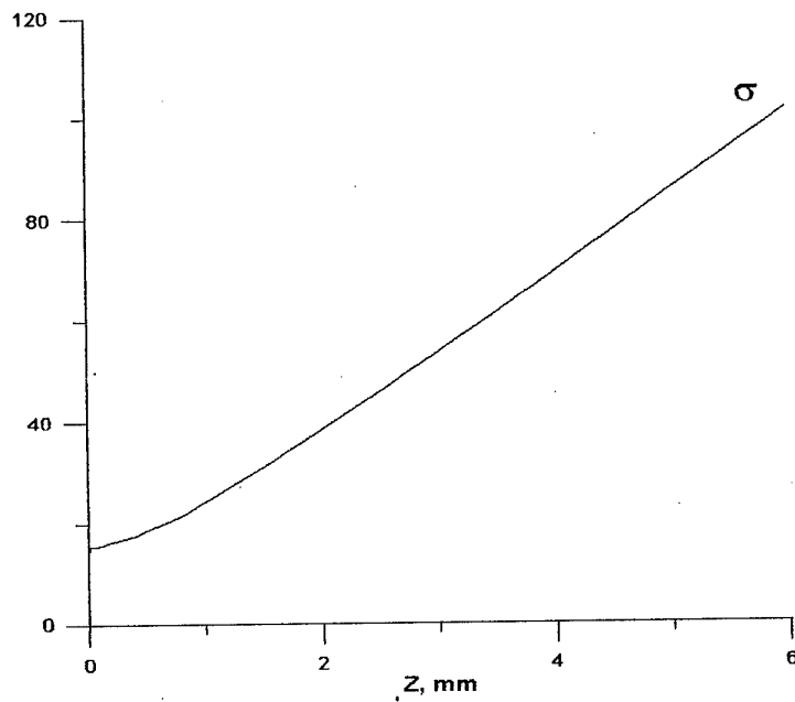
Fig. 3.8. Spatial distribution of plasma conductivity, 1/(\text{Ohm}\cdot\text{m}) , at T = 160 K, p = 70 Torr
