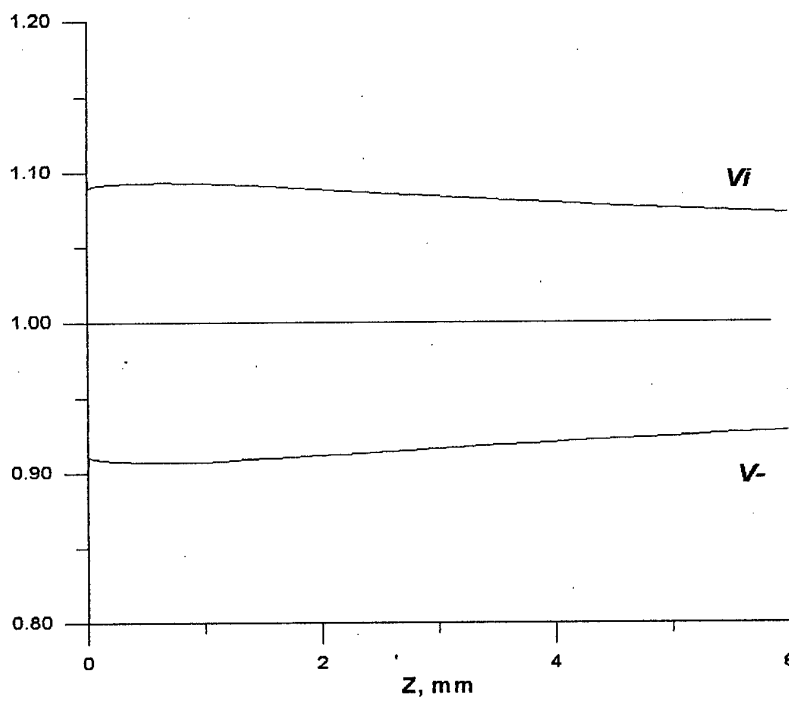
Fig. 3.12. Relative speed of positive and negative ions at T = 160 K, p = 70 Torr
