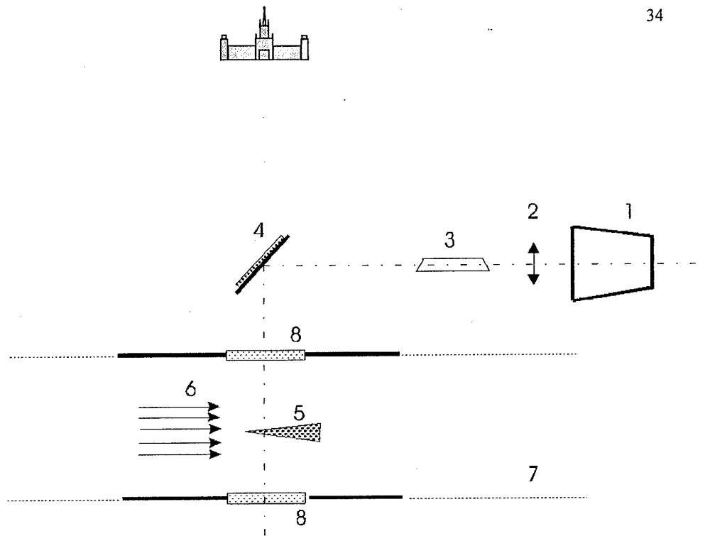
Fig. 2.15. A set up for spectral diagnostics of plasma in airflow: 1 - spectral device input slot, 2 - focusing quartz lens, 3 - prism, 4 - mirror, 5 - model, 6 - airflow, 7 - wind tunnel, 8 - window
