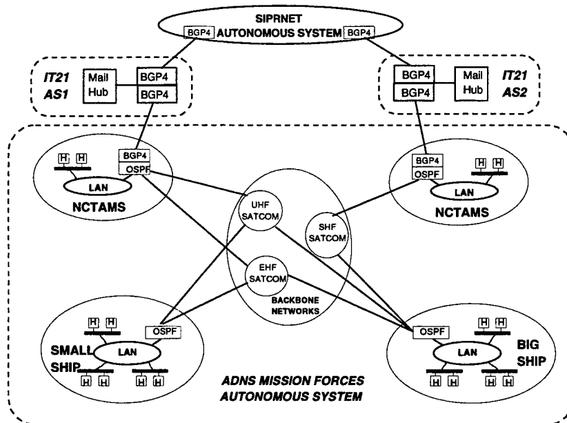
Figure 8. Generic ADNS AS Architecture. From Ref [Casey].
