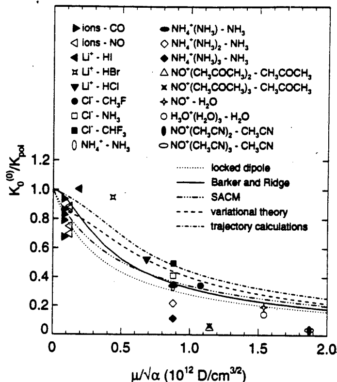
Figure 2. The ratio between the measured and calculated zero-field mobilities K_0^{(0)} and the polarization limit K_{pol} as a function of the parameter \mu/\sqrt{\alpha} at 300 K.
