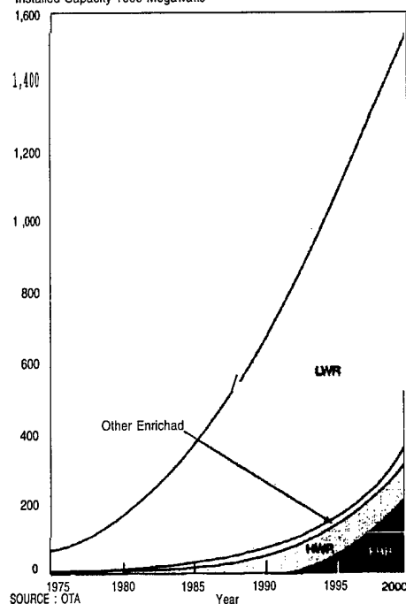
Figure x-12. World Nuclear Capacity Projection Installed Capacity 1000 Megawatts
