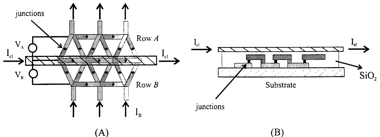
Figure 1: Schematic top view (a) and cross view (b) of a double row array made of 5 × 2 cells and with the control line.
