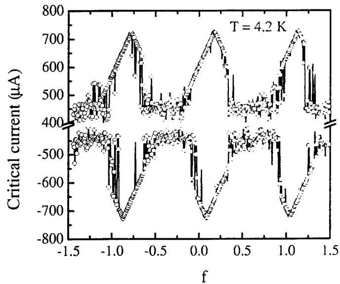
Figure 4: I_c(H) dependence at T = 4.2 \text{ K} for array 2897D#5.
