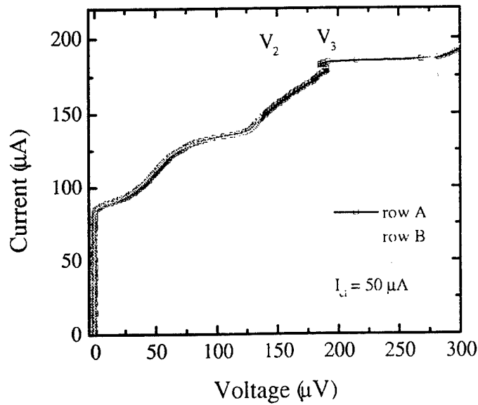
Figure 16: I - V curves of the two rows when a current I_c = 50 \mu\text{A} is passed in the control line.
