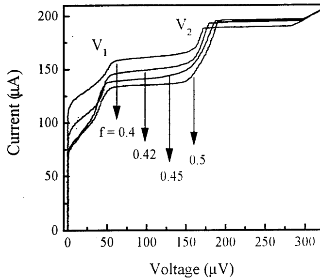
Figure 3: Overlapped I-V curves of one row array (sample 2897A#5) at different values of frustration f . When changing f , the lower step V_1 moves in the range 0 - 60 \mu\text{V} , the upper step V_2 moves in the voltage range 160 - 190 \mu\text{V} . Here the McCumber parameter \beta_c is \approx 500 .
