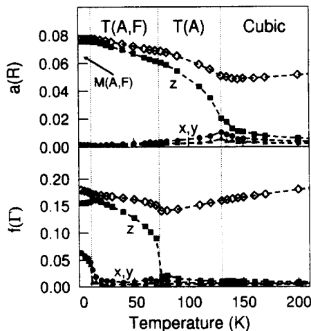
FIG. 2. Order parameters of \text{SrTiO}_3 vs T at P_0 = -5.4 GPa. Upper panel: averaged largest, middle, and smallest Cartesian components of a(R) . Lower panel: corresponding quantities for f(\Gamma) . Phase labels are the same as in Fig. 1.
