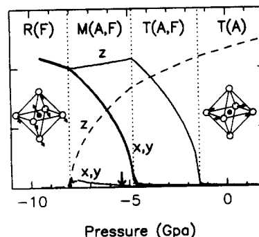
FIG. 1. T = 0 order parameters vs pressure for \text{SrTiO}_3 . Solid and dashed lines denote Cartesian components of f(\Gamma) and a(R) , respectively. Phases are labeled by lattice symmetry ( R = rhombohedral, M = monoclinic, T = tetragonal, O = orthorhombic) and by instabilities present ( A = antiferrodistortive, F = ferroelectric). Dotted lines denote phase boundaries. Vertical arrow indicates theoretical pressure P_0 at which the lattice constant matches the experimental P = 0 one. Left inset: sketch of displacements leading to R(F) phase (Sr is omitted for clarity). Right inset: same for T(A) phase.
