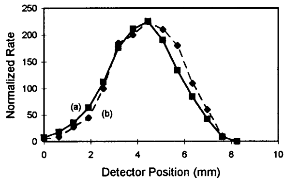
FIG. 3. The normalized rate of electron counts vs detector position for the cases of (a) thermal emission (TE) by counting single emission peaks and (b) field emission (FE) from harmonics above the fundamental, both originating from a W point filament. A 3 mm diam iris was used in measuring the FE and TE intensity profiles.
