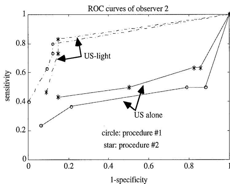
Fig.11. ROC curves measured with two different test procedures. (a) Obtained from observer 1, and (b) from observer 2. Procedure #1 is the ordered test with ultrasound and ultrasound-light images presented in sequence while procedure #2 is the random test with ultrasound and ultrasound-light images presented in random order. The results with both testing procedures are consistent.
