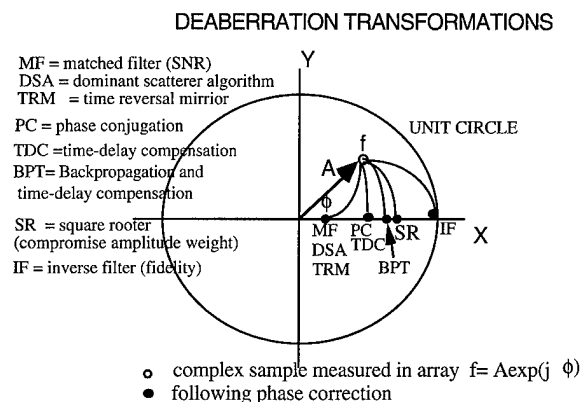
Figure 5. Deaberration transformations. \mathbf{f} is distortion vector for instantaneous sample of the radiation field. Transformations to the real axis all correct phase. Left (MF) maximizes SNR but increases amplitude distortion. Right (IF) maximizes imaging fidelity but increases noise. SR is a good compromise.
