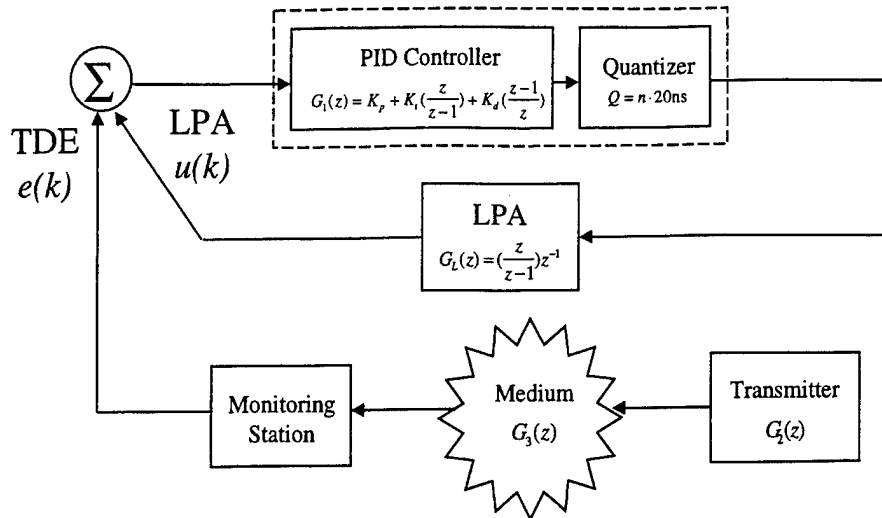
Figure 5: Simulation Model of the Loranc-C Control System.
