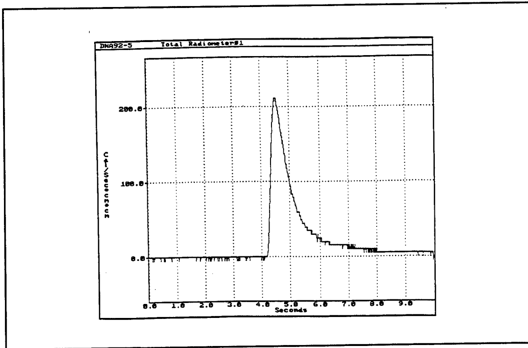
Figure A-4. Test DNA 92-5, total radiometer.
