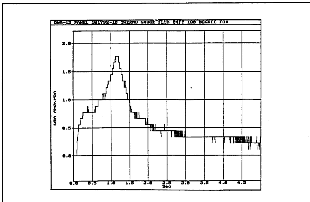
Figure C-22. thermogauge heat flux gauge, flux on detector, test #12.
