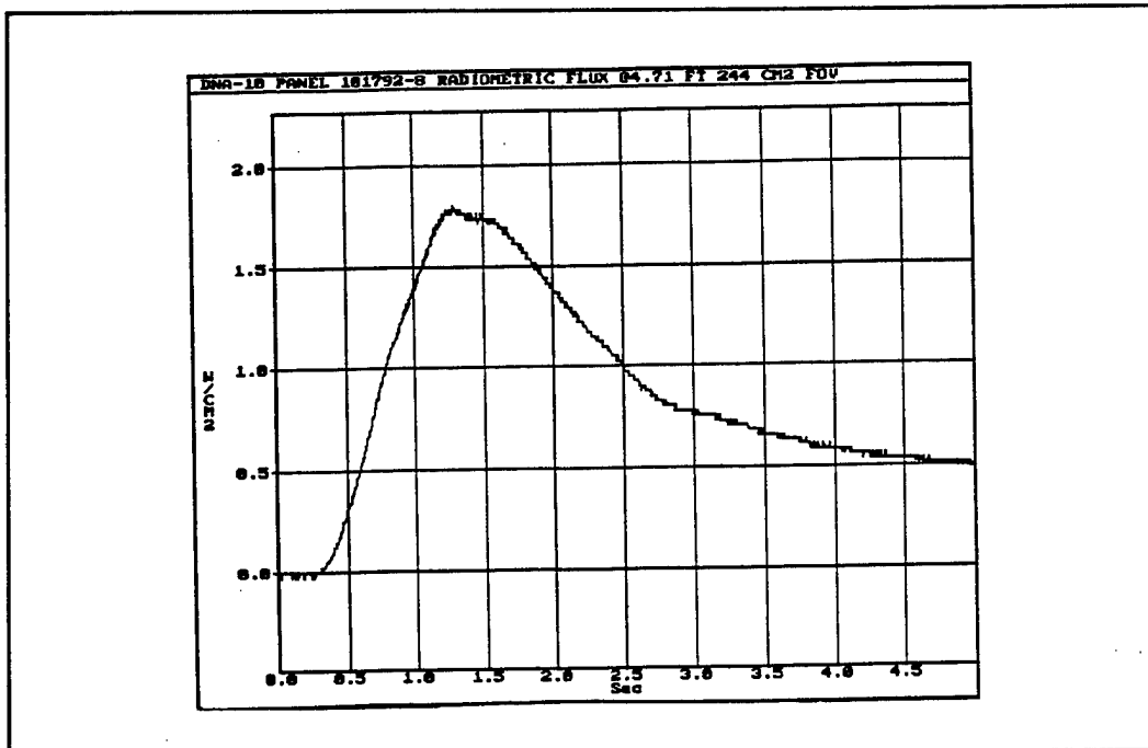
Figure C-19. Radiometer, flux on detector, test #10, uncorrected for FOV.
