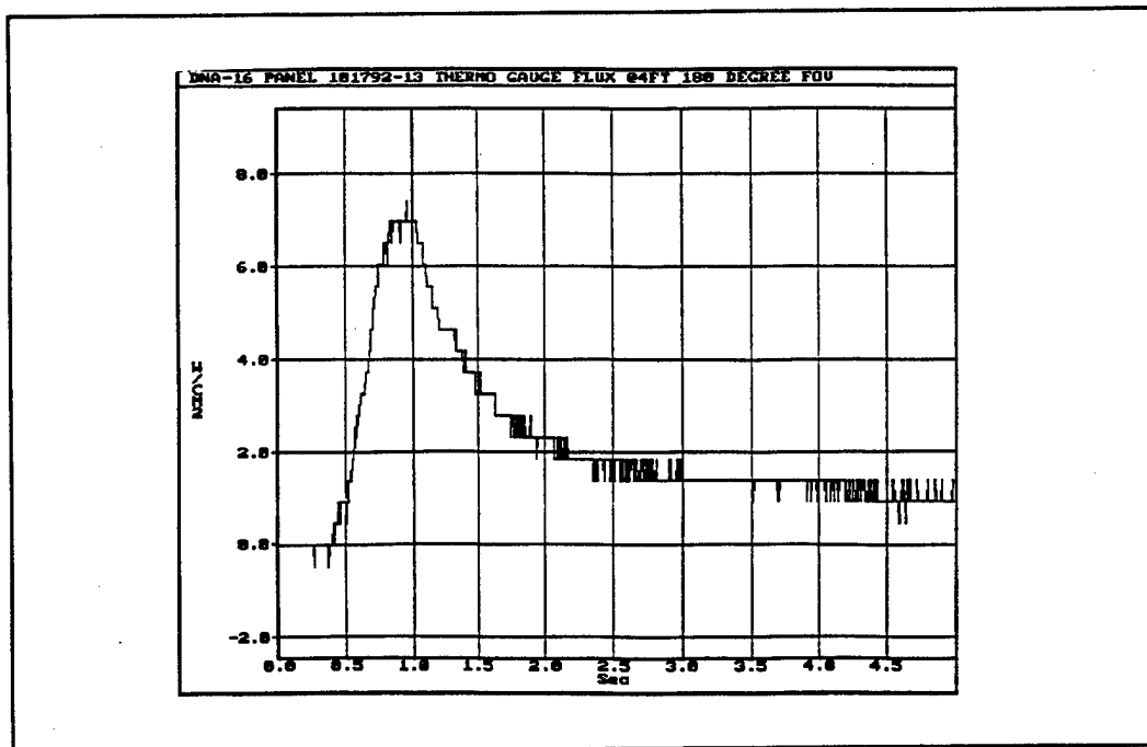
Figure C-28. thermogauge heat flux gauge, flux on detector, test #16.
