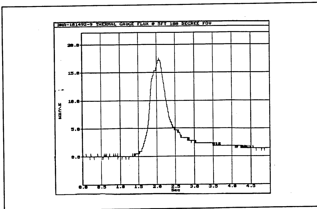
Figure C-18. thermogauge heat flux gauge, flux on detector, test #9.
