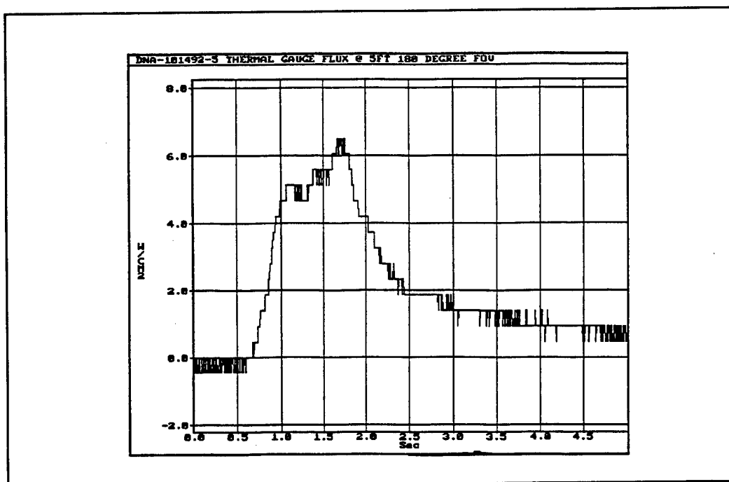
Figure C-10. thermogauge heat flux gauge, flux on detector, test #5.
