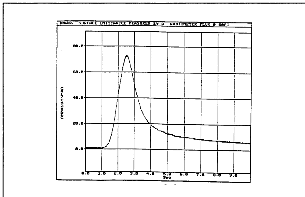
Figure A-15. Test DNA 92-36, total radiometer.
