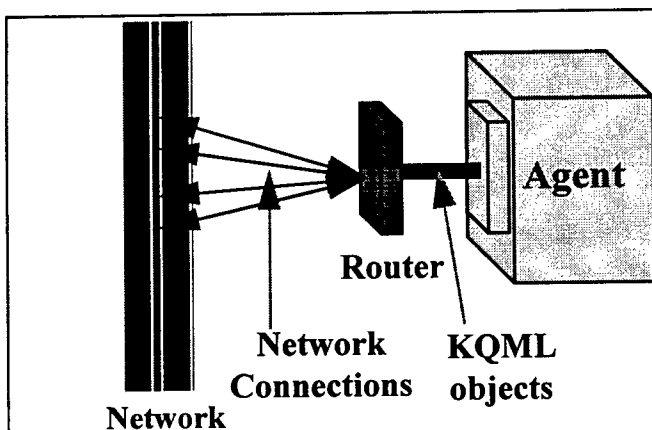
Figure 15. A router gives an application a single interface to the network, providing both client and server capabilities, managing multiple simultaneous connections, and handling some KQML interactions autonomously.
