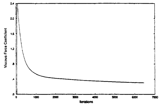
Figure B-20. NASTD Force Convergence History, Grid n-9
