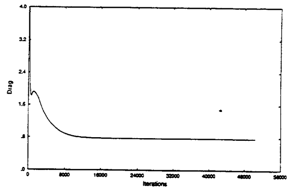
Figure A-28. Cobalt Force Convergence History, Grid c-8
