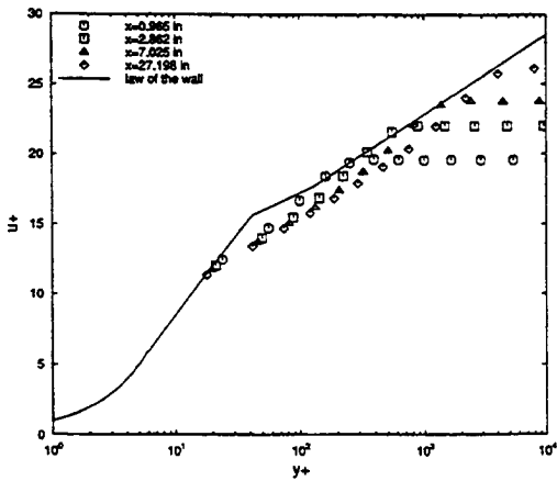
Figure 54. Velocity profile, USM3D turbulent solution, Mach 0.7, Re=12x10 6 , Grid u-1.
