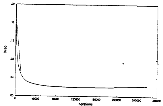
Figure A-16. Cobalt Force Convergence History, Grid c-8
