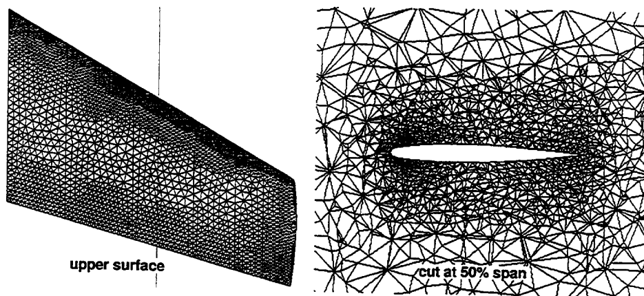
c) grid ne1 (15,279 surface faces, 231,507 tetrahedra)
