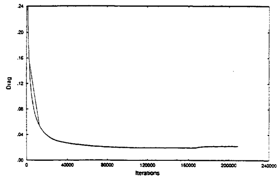
Figure A-14. Cobalt Force Convergence History, Grid c-7
