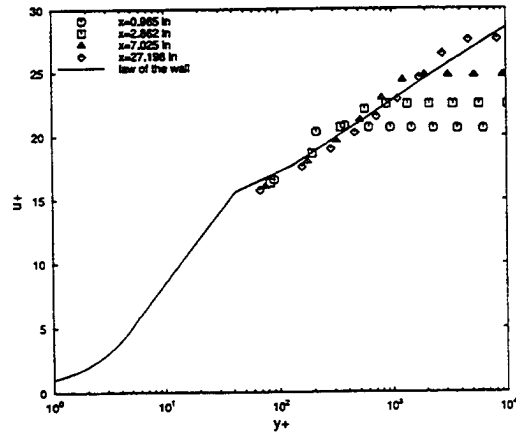
Figure 55. Velocity profile, USM3D turbulent solution, Mach 0.7, Re=12x10 6 , Grid u-6.
