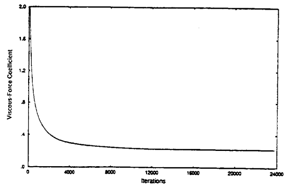
Figure B-18. NASTD Force Convergence History, Grid n-8
