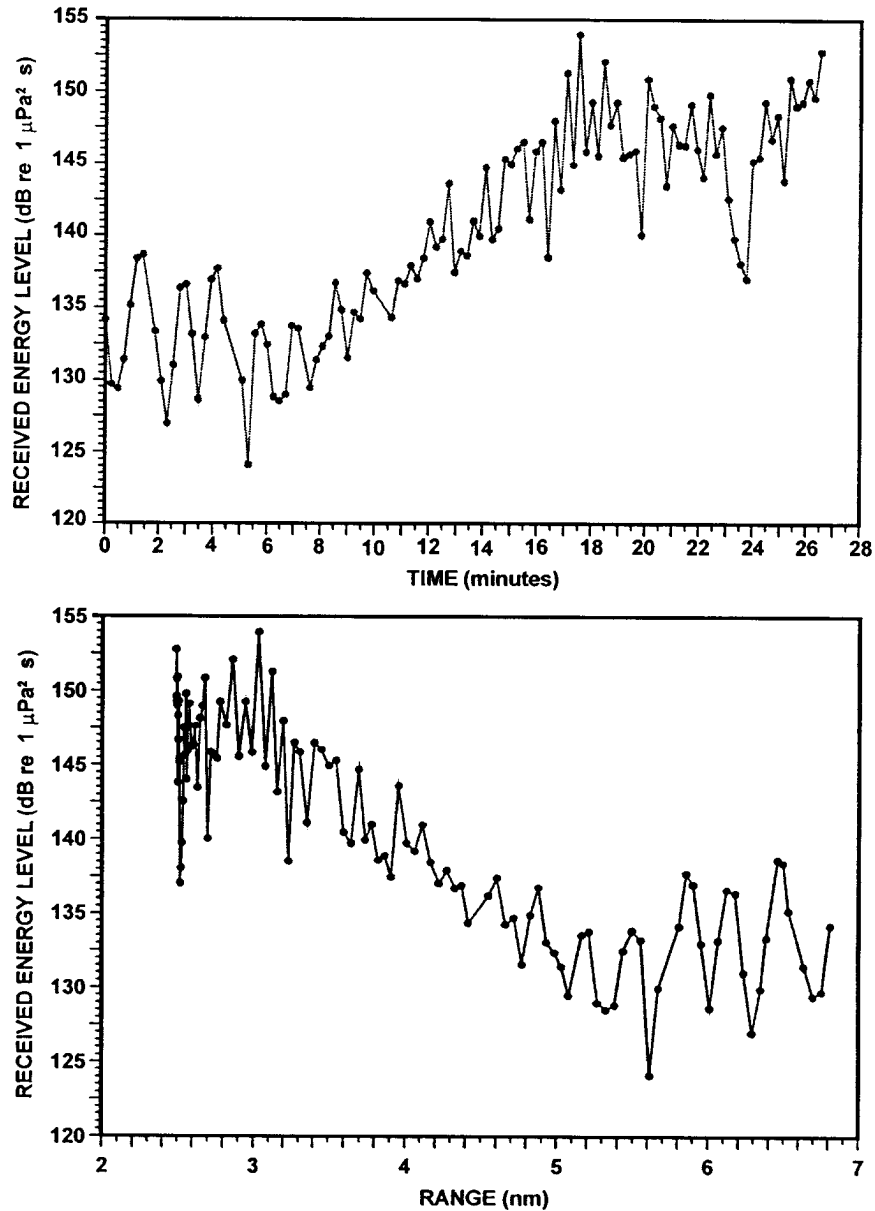
Figure 14: Received energy level for U.S.S. Nicholson SQS-53C LFM signal as a function of time and range to receiver. Start time was 1725 hours (Z) on 14 September 1997.
