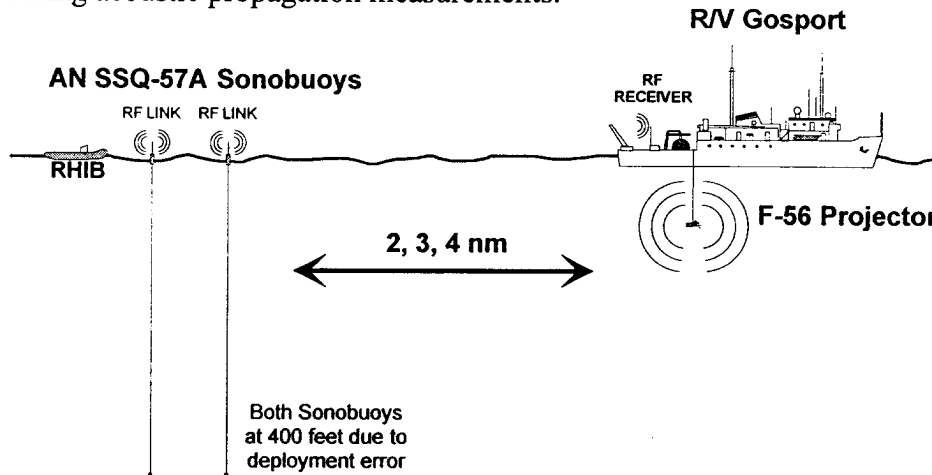
Figure 2: Measurement configuration for the acoustic propagation measurements performed at sites ZL and ZLS.
