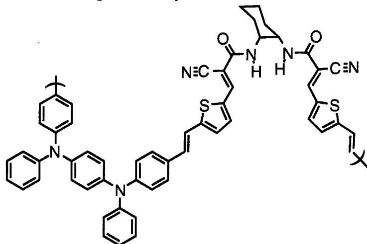
Figure 2: High Glass Transition Nonlinear Optical Polymer
