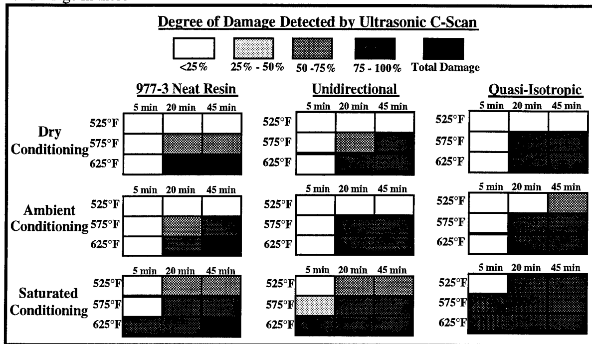
Figure 4. Degree of Damage Detected by Ultrasound
