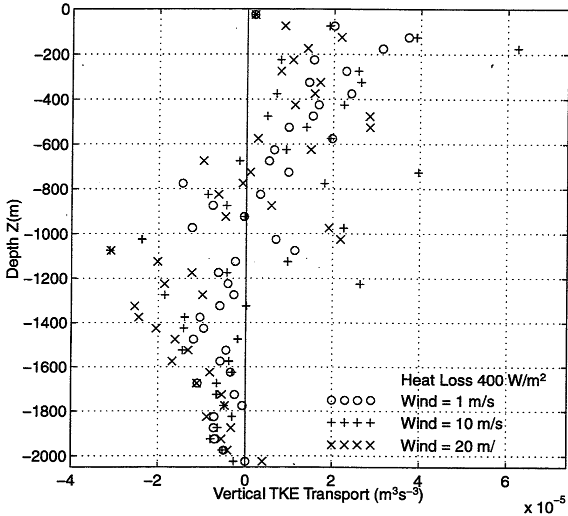
The Vertical TKE Transport Observed by Isobaric Drifters
