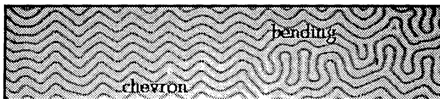
Picture 1 : chevron and bending patterns are obtained at the same threshold value of the magnetic field in the same system (the period of the layers is roughly 3 mm).
