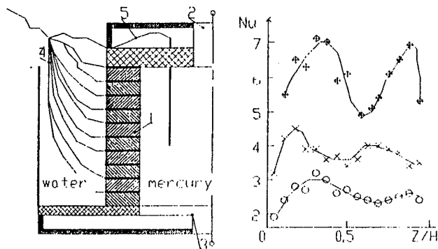
Fig.1. Physical model of electroslag furnace.
