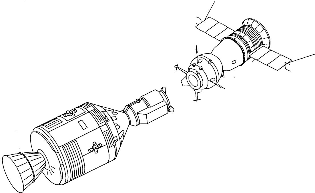
FIGURE 3-1: Apollo and Soyuz Join in Space
