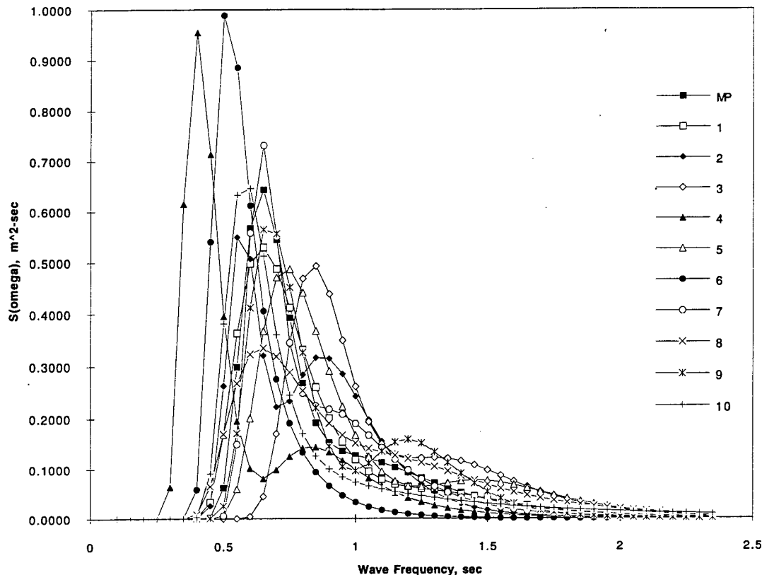
Figure 12. Ochi-Hubble 6-parameter spectral family for a mid Sea State 4.
