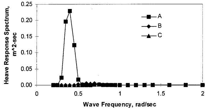
Figure 9. Heave response spectra of a large floating platform for Wave Spectra A,B and C.
