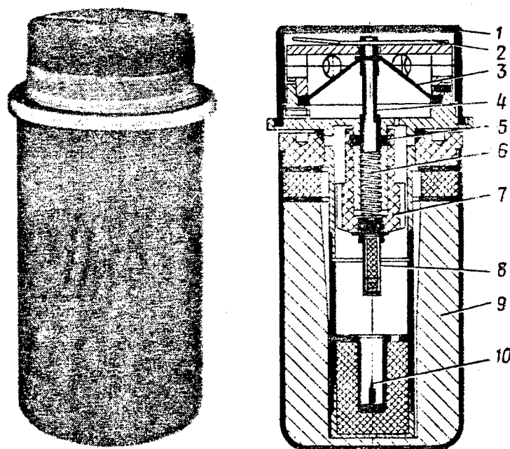
Fig. 5. Overall view and design of LM-2 demolition charge: 1--Safety cap; 2--Safety pin; 3--Conical diaphragm; 4--Stem; 5--Retaining ball; 6--Striker spring; 7--Bushing; 8--Igniter; 9--Explosive charge; 10--Firing pin.
