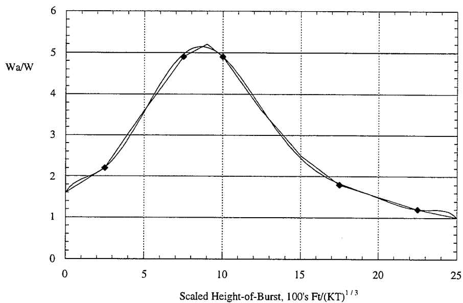
Figure 12. The ratio of the equivalent yield, free air burst, W_a to the chemical yield, W , as a function of the scaled height-of-burst. [Figure based on data provided by Reed (1969).]
