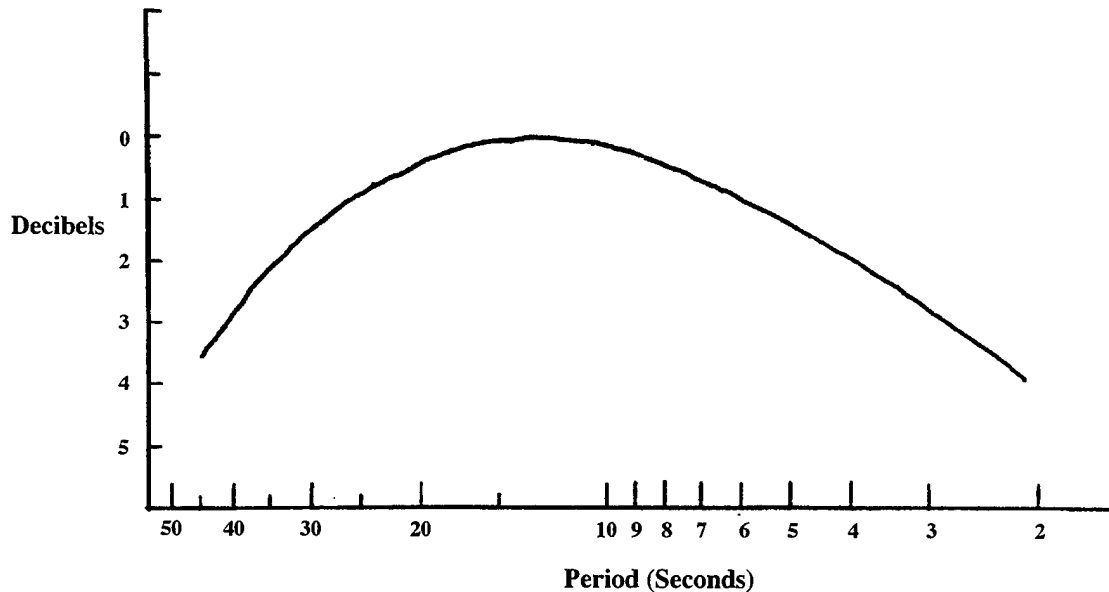
Figure 3. The frequency response of the improved infrasonic system M-2. [Figure adopted from Crenshaw, Lonnie and Pressman (1952) .]
