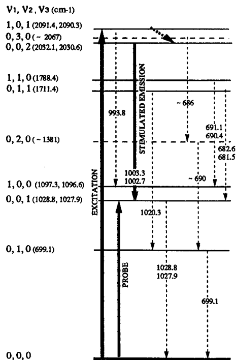
Energy levels of O 3 in xenon matrix
