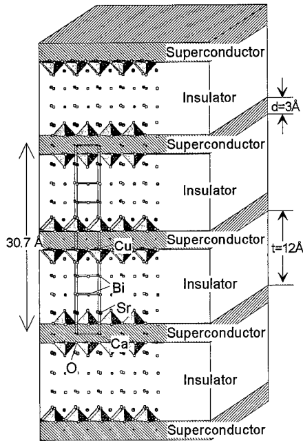
Fig. 2. Superposition of the lattice structure of \text{Bi}_2\text{Sr}_2\text{CaCu}_2\text{O}_8 with the stacking sequence of the model.
