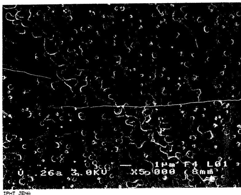
Fig. 1. SEM top view of a TBCCO thin film on a step edge \text{LaAlO}_3 substrate ( step slope 30° )
