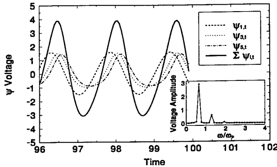
Fig. 6. Plot of \psi_i(x = L, t) voltage amplitudes and frequencies with random J_{c0} defects of \pm 60\% for N_J=6 , B_T=4 , L=20 , I_{bc}=1.1 , \eta=1 and \alpha = .25 . Inset: Amplitude of Fourier transform of \sum \psi_{i,t} vs. frequency.
