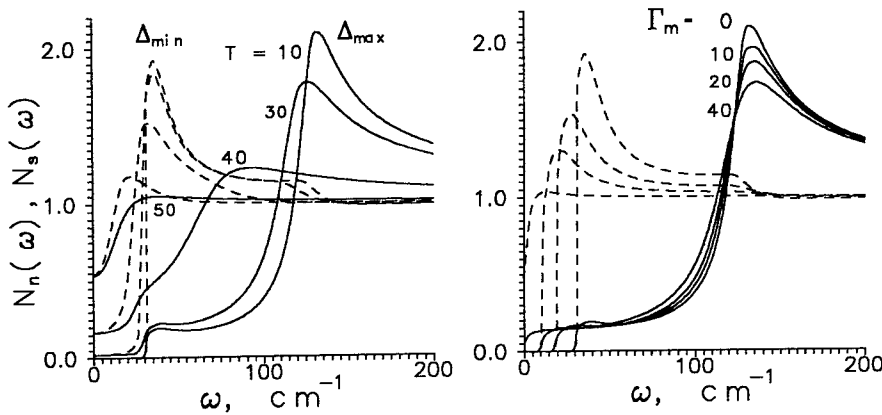
Fig. 2. Left: DOS in s-band (solid lines) and in n-band (dashed lines) at various temperatures T (in cm^{-1} ). Right: the same for various \Gamma_m (in cm^{-1} ) at T = 10
