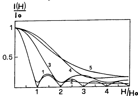
Fig. 2. Numerical results for the one-dimensional case: 1) a=L , \sigma = 0 ; 2) a=L , \sigma = 0.1 ; 3) a=0.5L , \sigma = 0.1 ; 4) a=0.3L , \sigma = 0.2 ; 5) a=0.3L , \sigma = 0.5
