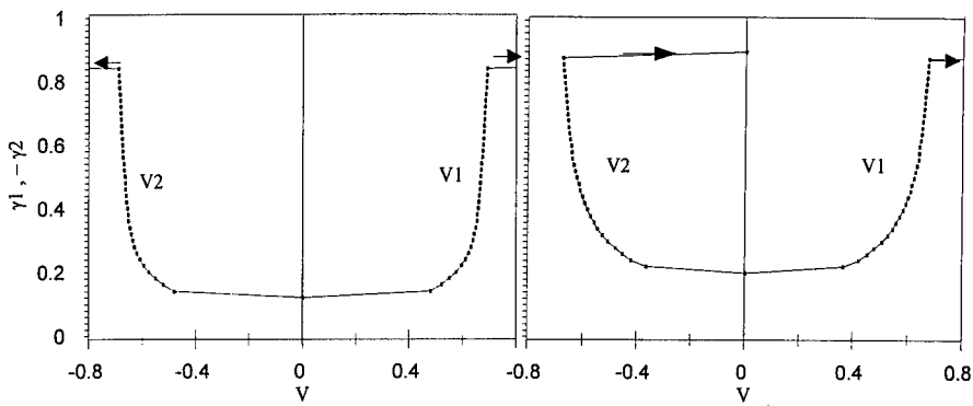
Fig. 3. I-V curves for a stacked junction in the ZFS state. Parameters: \alpha = 0.1 , l = 7.0 , S = 0.7 . V_1 = \langle \varphi_t \rangle , V_2 = \langle \psi_t \rangle . (a) \gamma_1 = -\gamma_2 ; (b) \gamma_2 = 0 .
