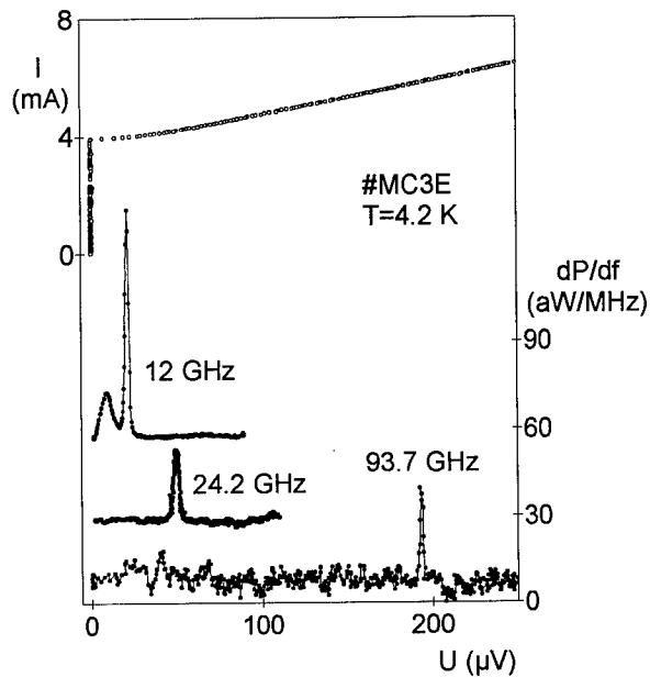
Fig. 2. I-V characteristic of an YBa_2Cu_3O_{7-x} biepitaxial junction (left scale) and microwave power at three different detection frequencies (right scale). The zero of the three emission measurements is offset by 30 aW/MHz each. Note the second harmonic at the lowest frequency.
