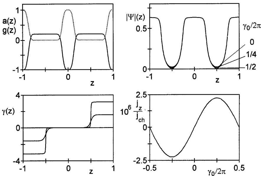
Fig. 3. Ginzburg-Landau model of a strongly modulated superconducting structure ( a_0 = 0.2 , a_1 = -1 , g_{\min} = 0.001 ). The superconducting electrodes are located at z = 0 and z = \pm 1 . 3a: Condensation and effective mass parameters a(z) (dotted line) and g(z) (upper left). 3b: Order parameter at different phase differences between the layers (upper right). 3c: Continuous phase difference vs. z (lower left). 3d: Current-phase relation (lower right). j_z is normalized to the pairbreaking critical current density j_{ch} .
