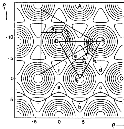
Fig. 2. Contour plot of the potential energy U(\rho_1, \rho_2) for an N=3 system (with \Phi = \Phi_0/2 ) with superimposed parametric plot of \psi(= \rho_1/2\sqrt{2}) vs. \theta(= \rho_2/\sqrt{2}) centered around \psi = +\pi/2 .
