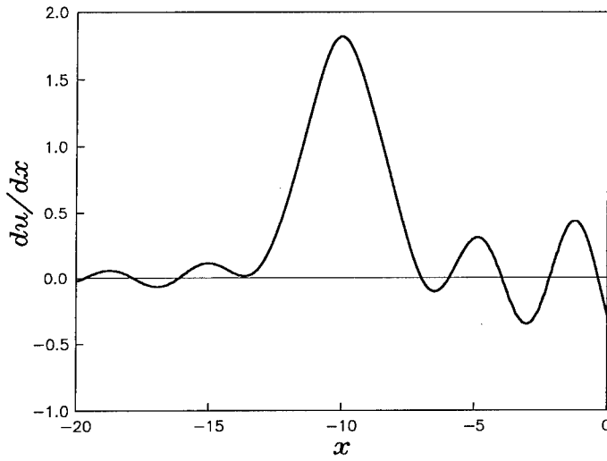
Fig. 1. A static fluxon interacting with a plasma wave in a long junction. \alpha = 0.2 , a = 0.5 , \omega = 2 .
