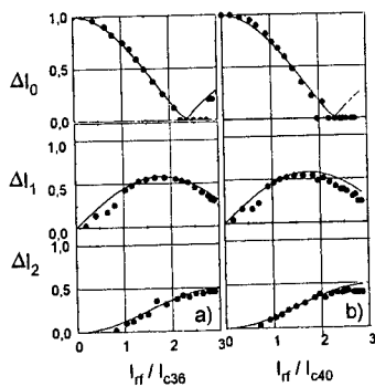
Fig. 15. Shapiro-steps height (with n = 0, 1, 2 ) as a function of rf current at f_{\text{ext}} = 79 \text{ GHz} for junctions JJ_{36} (a) and JJ_{40} (b). Continuous curves described by (1).
