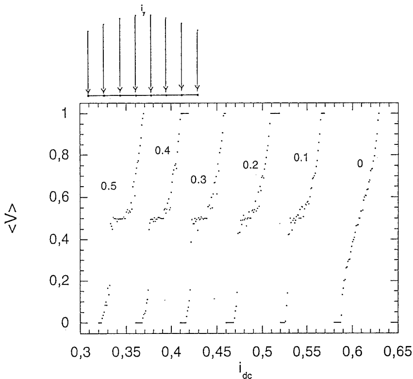
Fig. 1. I-V plot for a 7 \times 7 array with non uniform injected current. This has the form i_{ext}(x) = g(x)[i_{dc} + i_{ac} \sin(2\pi\nu t)] , where g(x) = 1 + \Delta i * \sin(\pi x / N p_x) ( N p_x is the number of plaquettes along the x axis, in this case equal to 6). \Delta i varies from 0 \rightarrow 0.5 .
