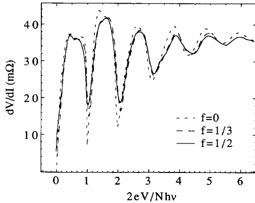
Fig. 7. Differential resistance as a function of the normalized voltage for three different frustrations in an array oriented in the [11] direction.
