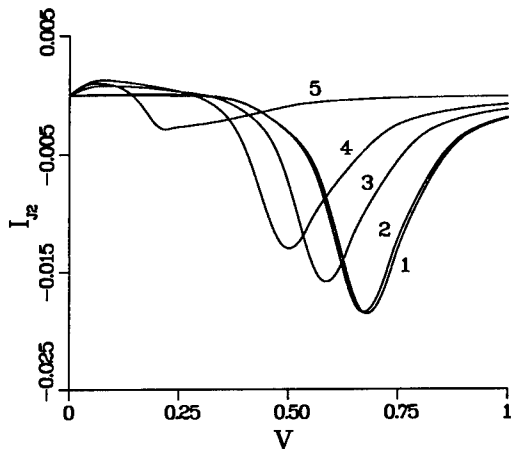
Figure 3: The supercurrent I_{J2} at various temperatures 1: T=0.0 , 2: T=0.05 , 3: T=0.10 , 4: T=0.12 , 5: T=0.15 .
