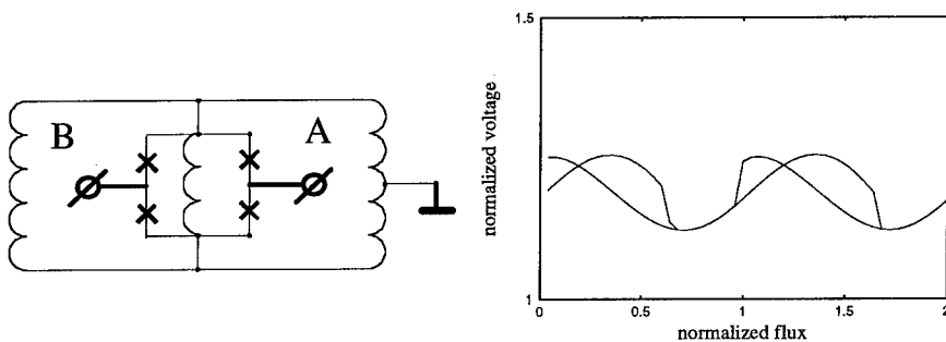
Fig. 8. a) Circuit of a DC-SQUID gradiometer containing two SQUIDs in the middle of the structure, b) Calculated flux-voltage dependence in the case that second SQUID is not cut off ( I_{C1} = 0.1I_{C2} )
