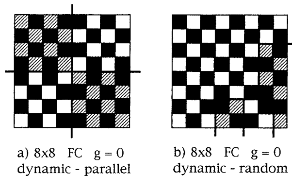
Fig. 4 - Vortices configurations at f = 0.5 obtained following a a) FC dynamic procedure with g = 0 and phases initially aligned; b) FC dynamic approach with g = 0 and phases initially random distributed; these two configurations settled on firmly respectively after 200 \tau and 300 \tau with \tau = h/2eR_c
