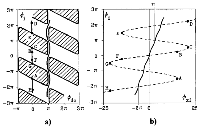
2. Operating regime "a": a) stable steady states domain D ( unshaded areas ); a) and b) the operating point trajectories for different coordinates when the signal flux is an integer of flux quantum (capital letters, dashed line), and a half integer of flux quantum (solid line).
