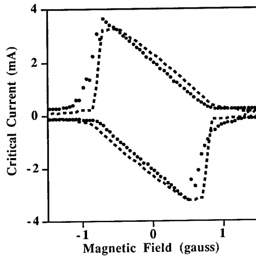
Fig.3 Magnetic field dependence of the critical current for the device proposed. The dots are experimental results of a 1000+300\ \mu\text{m} long junction, and the dashed curve is the result of the numerical simulation (see text for details).
