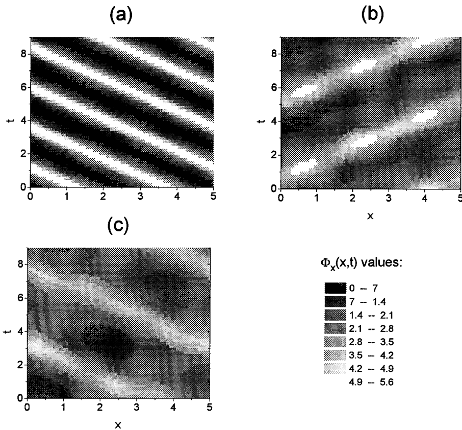
Fig. 3. The spatio-temporal evolution of \varphi_x(x, t) corresponding to different points of the current-voltage characteristic shown in Fig. 2 : (a) point A; (b) point B; (c) point C. The values for \varphi_x are given in grey scale.
