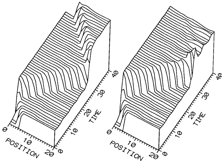
Fig.5 Numerical simulations of the phase evolution for a constant width (left), and a narrowing width (right) junction. The values of the parameters are: \alpha=0.02 , \beta=0 , \gamma=0.3 , u(0) = -0.9964 , L=20 , L_T=10 . w_1/w_0 = 1 , Z_j/Z_T = 0.1 (left) and w_1/w_0 = 0.1 , Z_j/Z_T = 1 (right).
