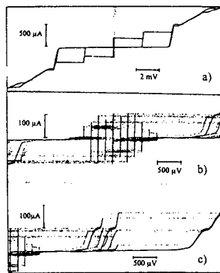
Fig. 16. I - V curve of the two junction stack (a). Shapiro steps at f_{\text{ext}} = 79\text{ GHz} in the vicinity V = 0 (b) and V = V_g (c).
