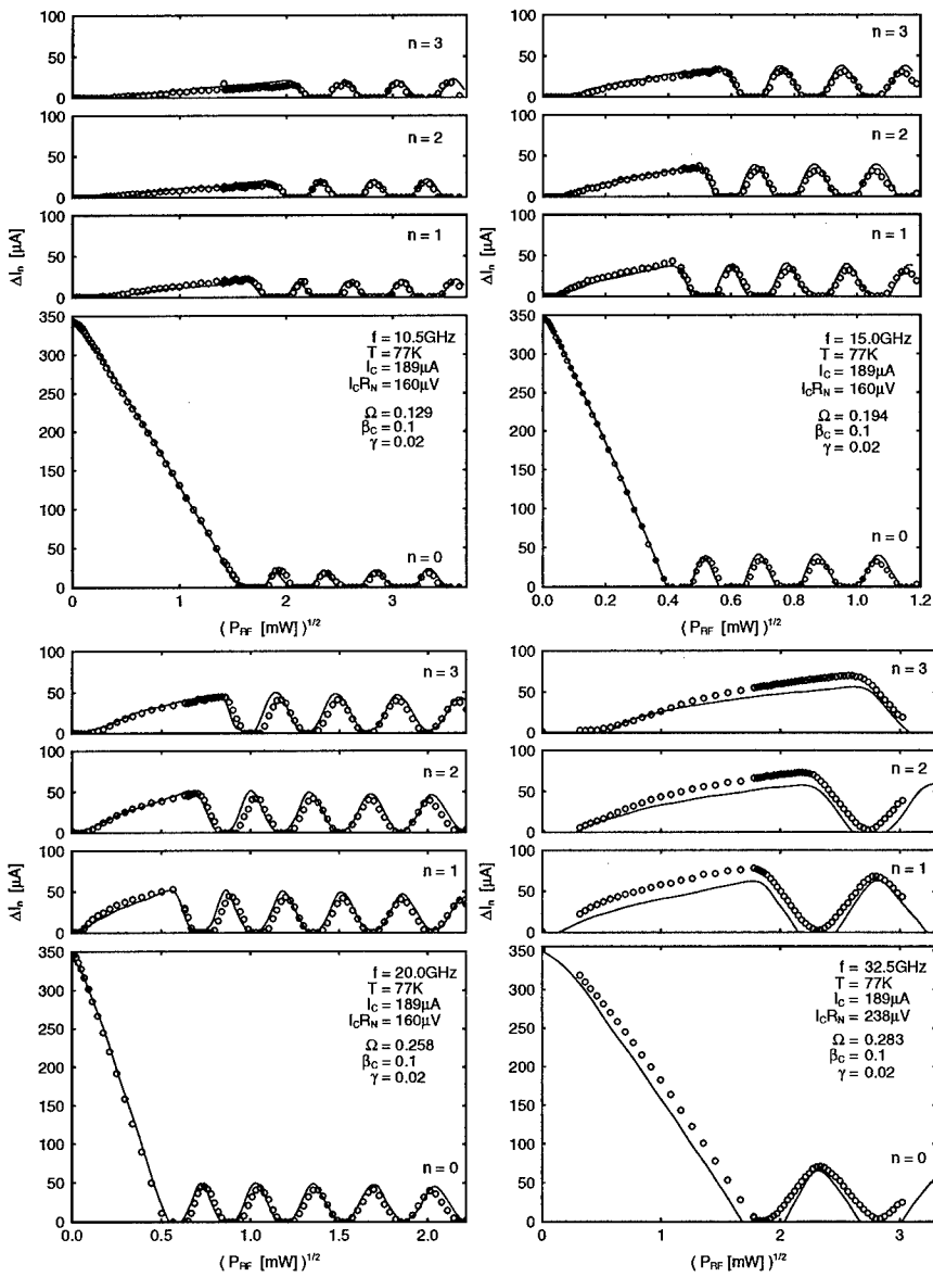
Fig. 3. Heights of Shapiro steps vs. RF amplitude for an YBCO bicrystal junction at T = 77\text{K} for different microwave frequencies
