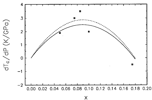
Fig. 3. The pressure derivative of critical temperature as a function of composition x in \text{La}_{2-x}\text{M}_x\text{CuO}_4 compound. Solid line corresponds to \tilde{\delta}' = -80 , dashed line to \tilde{\delta}' = -90 ; bulk modulus is B = 180 GPa. The experimental data are taken from Ref. 12.
