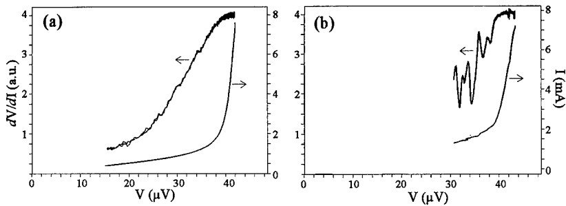
Fig. 7. dV/dI - V and I - V curves for ZFSIs in junctions with W' = 2.5 \mu\text{m} (a) and W' = 30 \mu\text{m} .
