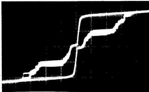
Fig. 13. I - V curve an array with (4 \times 5) junctions under 70\text{ GHz} irradiation. Horizontal: 50\text{ A/div.} ; Vertical: 20\text{ mV/div.}
