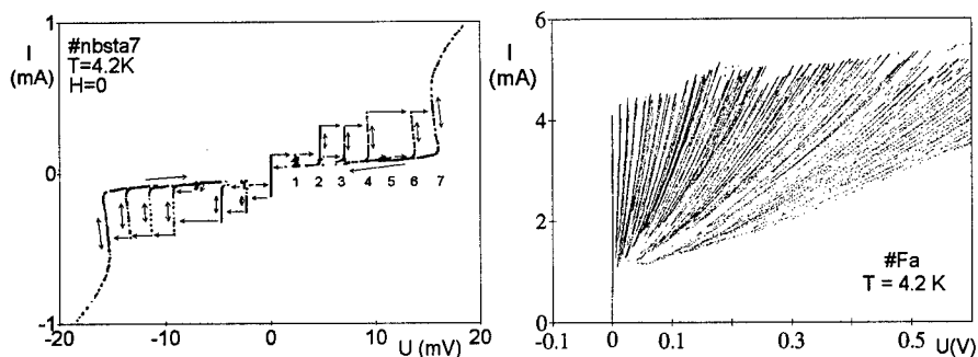
Fig. 6. Left part: I-V characteristic of a stack of 7 Nb/Al-AIO x /Nb tunnel junctions. The arrows mark the succession of data points produced by increasing or decreasing the bias current. The branch index corresponds to the number of junctions in the resistive state. Asymmetry and missing branches are caused by trapped flux. The backbending of the higher-order branches is due to quasiparticle injection.
