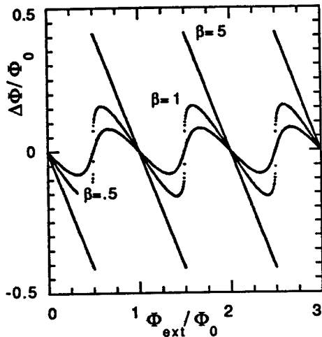
Fig. 1. \Delta\Phi vs. \Phi_{ext} curves calculated for different values of the SQUID parameter \beta = 2\pi LI_0^0/\Phi_0 and N = 1 . When \Phi_{ext} is in the range n\Phi_0 > \Phi_{ext} > (n - 1/2)\Phi_0 the internal flux is larger than the applied flux. This effect is larger for increasing \beta(T) .
