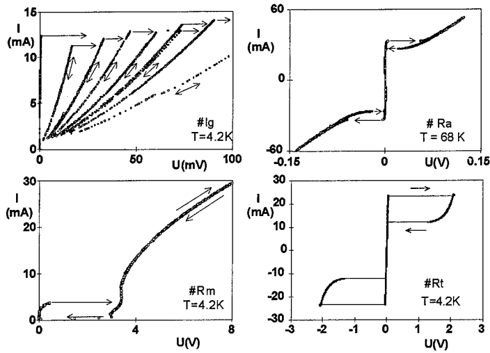
Fig. 7. Overview of different types of I-V characteristics. Left part: An annealed \text{Bi}_2\text{Sr}_2\text{CaCu}_2\text{O}_8 single crystals on different voltage scales. The single branches of the upper part are not traced out in the lower part. Note the quasiparticle-like characteristic at high voltages. Right part: Ideal RSJ characteristic of a Pb doped sample (upper half). Abrupt switching of a strongly hysteretic I-V characteristic (lower half). The contact resistance is not corrected here.
