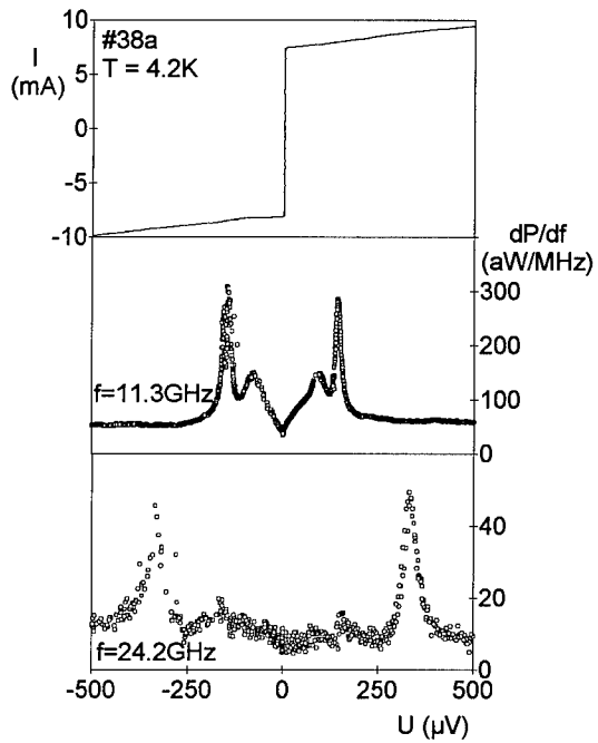
Fig. 7. I-V characteristic of a Tl (2223) thin film step stack at T = 4.2 K (upper panel), detected microwave power at f = 11.3 GHz (middle panel) and detected microwave power at f = 24.2 GHz (lower panel).
