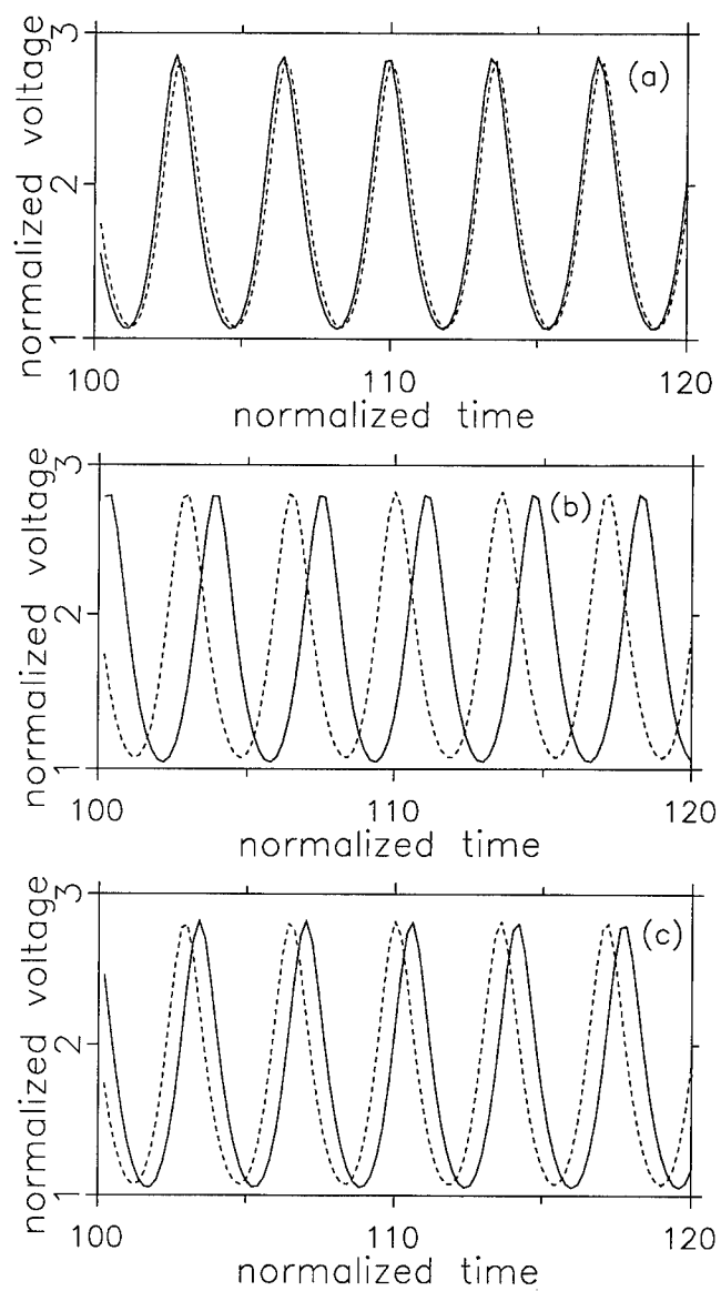
Fig. 4. Time evolution of the instantaneous voltage for the upper (solid line) and lower (dotted line) vertical junctions in the same column for a) \delta_1^Y = 0 , b) \delta_1^Y = 0.05 and c) \delta_1^Y = 0.03 . Parameters of the simulations are: M = 3 , N = 10 , l = 5 , \beta_l = 1 , \eta = \pi/4 , \gamma = 2 .
