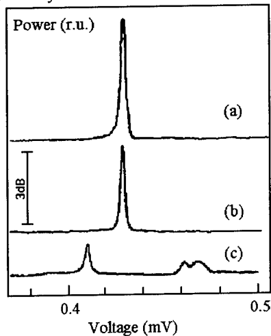
Figure 17. Detected power vs. voltage for a three-SQUID array in the presence of an applied magnetic field B . (a) B=0.0 , (b) B=3.0 , and (c) B=21.0 in relative units. f_{LO}=69.5\text{GHz} , T=4.2\text{K} .
