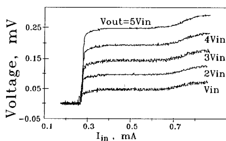
Figure 21. Experimentally obtained voltages on each stage of parallel QDVA vs. bias current of the input junction.
